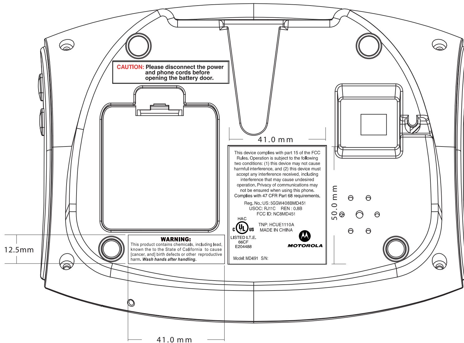
MD491 LABELLING DRAWING DATE: 10 MAR, 2004
