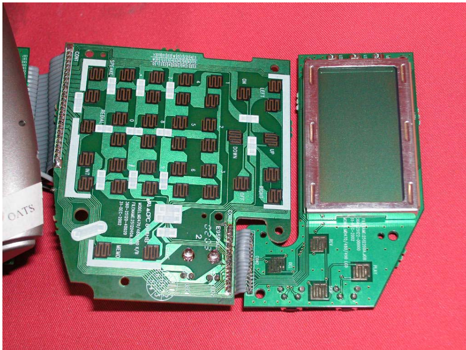
Base keypad and DAM PCBs front side
