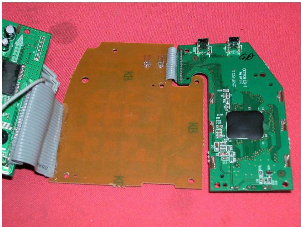
Base keypad and DAM PCBs rear side
