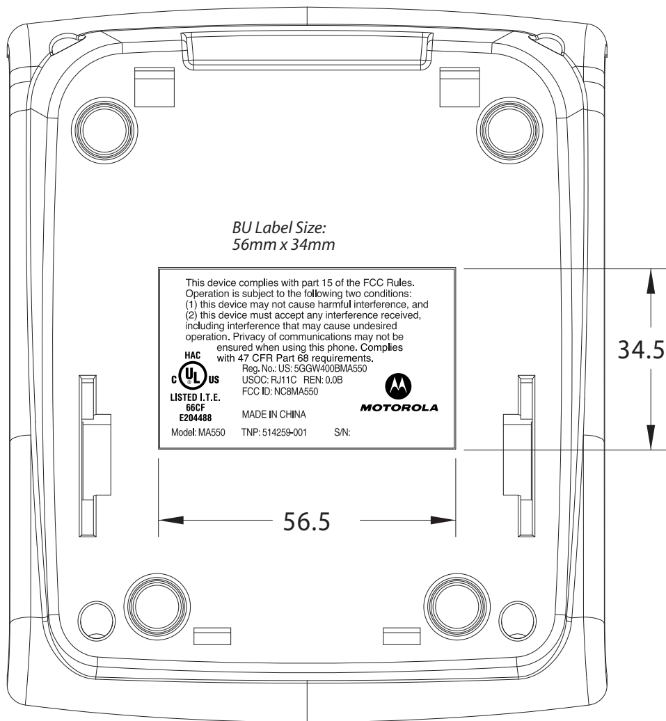
MA550-USA LABEL DRAWING DATE : 25 MAY 2004
