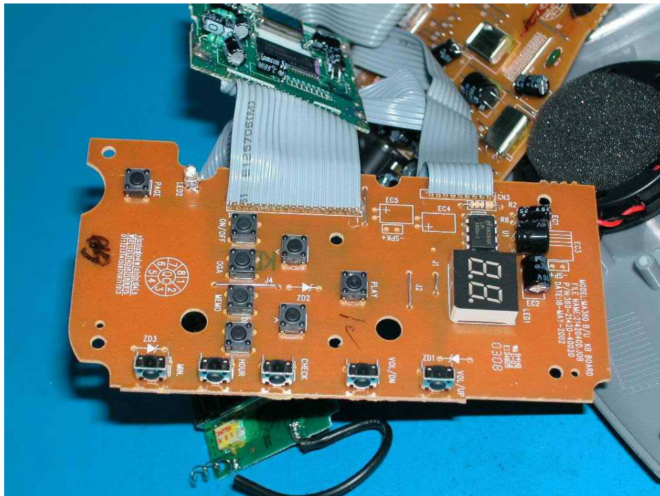
Base Answering Machine keypad front side
