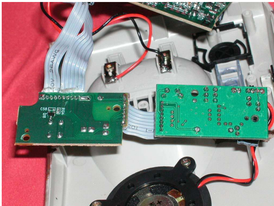
Base page key and melody key PCB solder side
