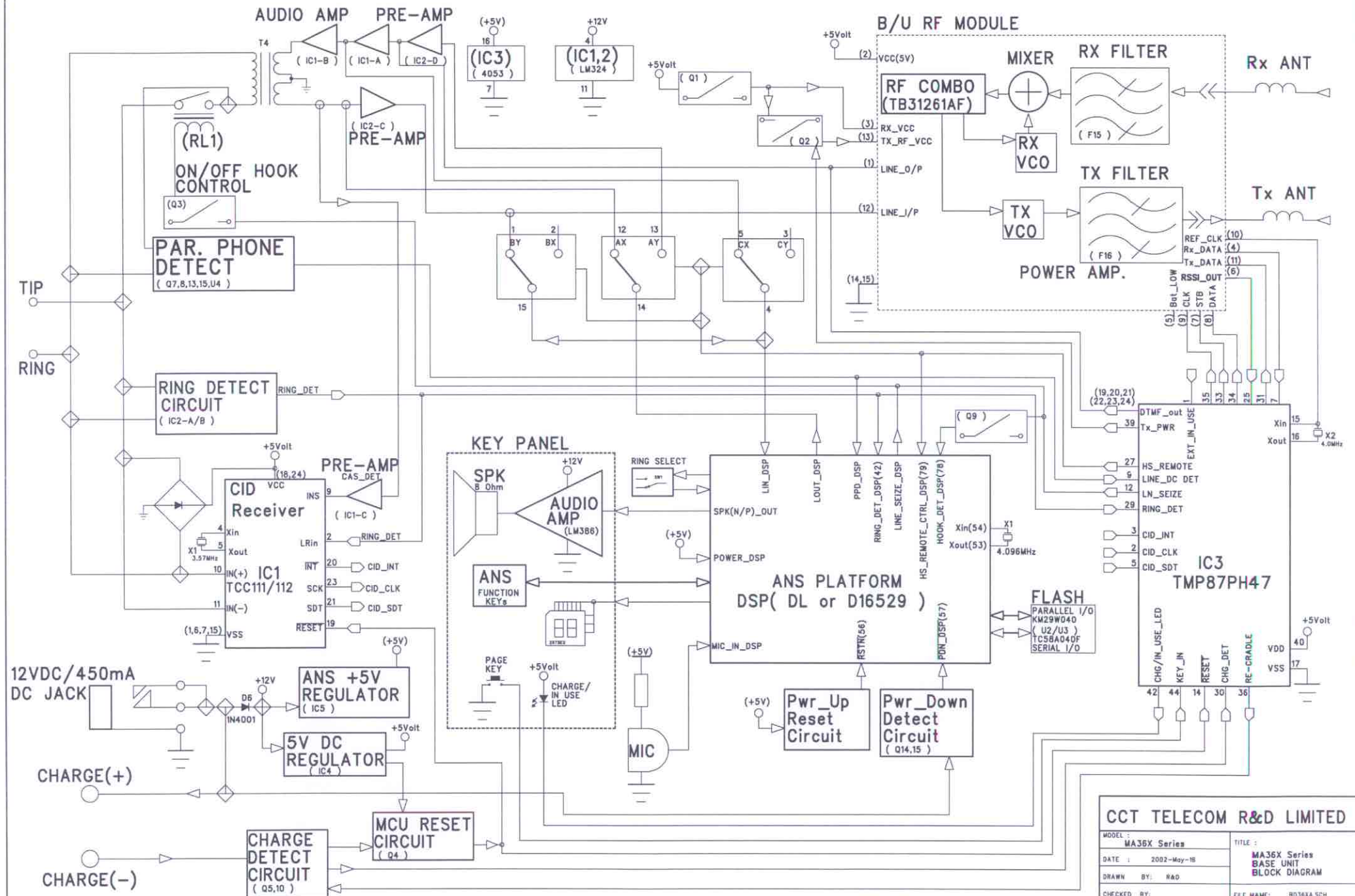
Base Unit Functional Block Diagram of MA36X
