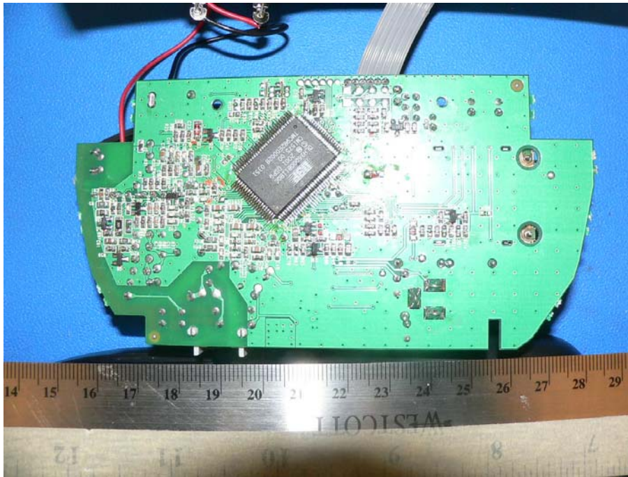
EUT – PCB Solder Side View (Base)
