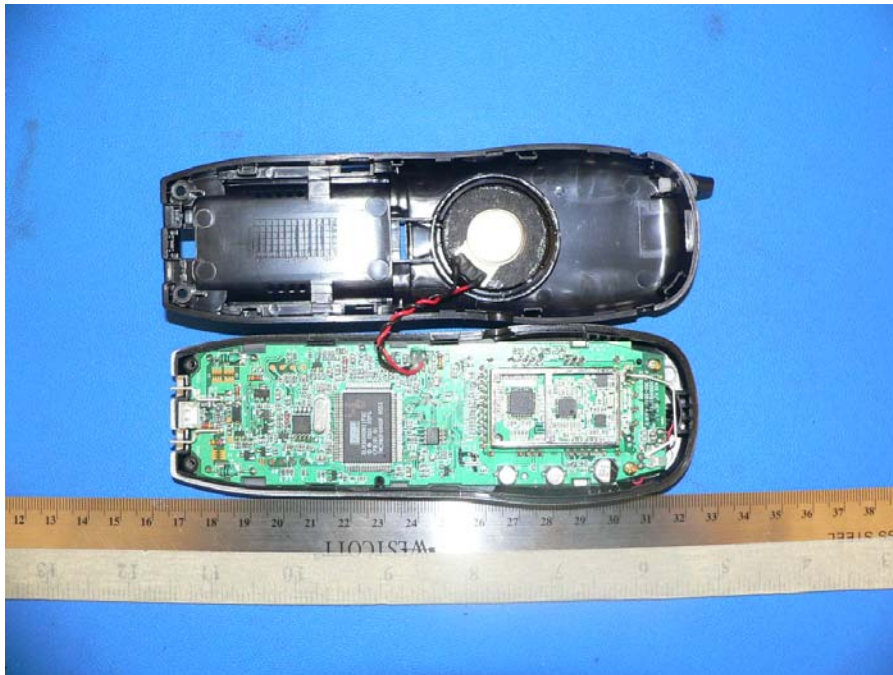
EUT –Chassis off View 1 (Handset)
