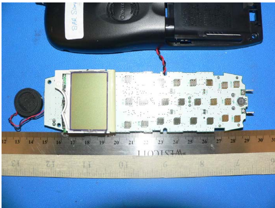
EUT – PCB Bottom Side View (Handset)
