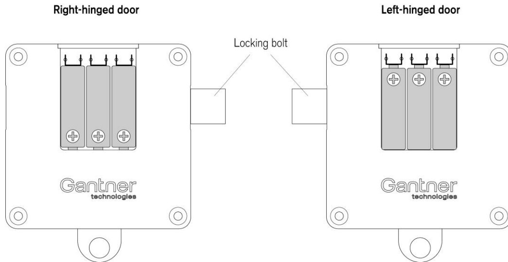
Figure 4.2 – Correct battery polarity
