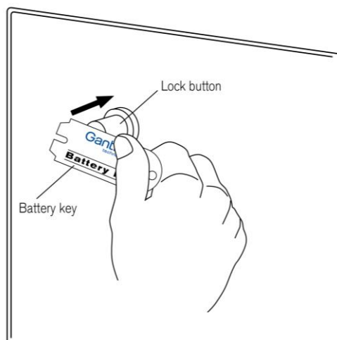
Figure 4.3 – Activating the GAT ECO.Lock with the battery cover key
