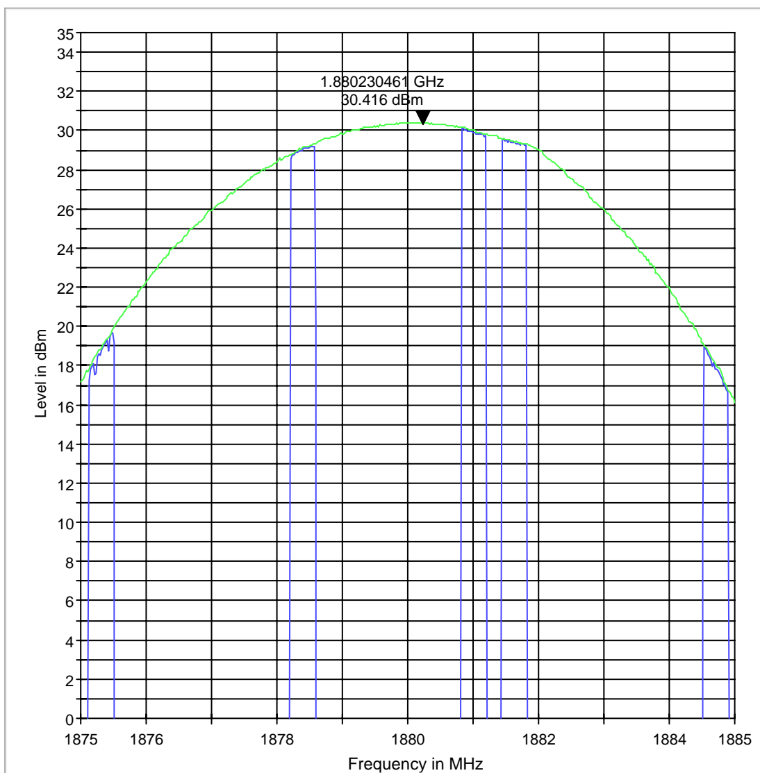
EIRP 1900 M
