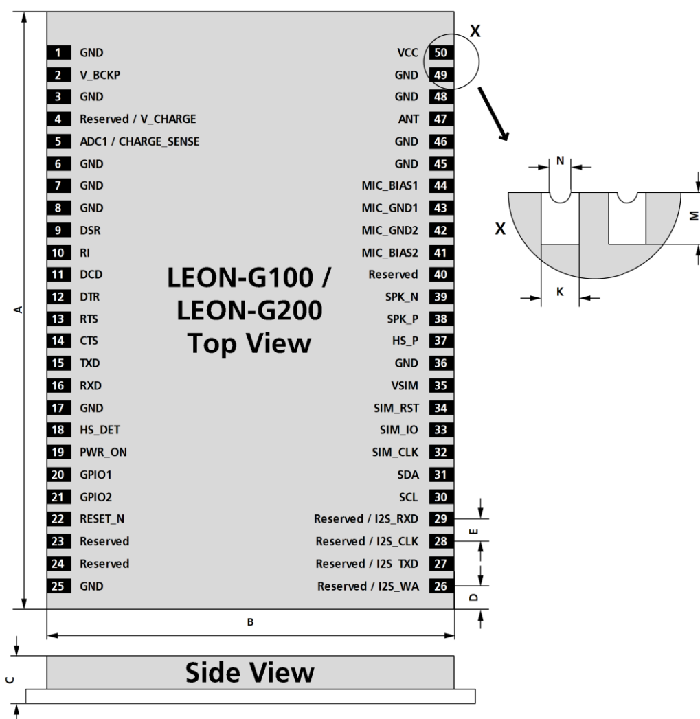
Figure 4: Dimensions and pinout
