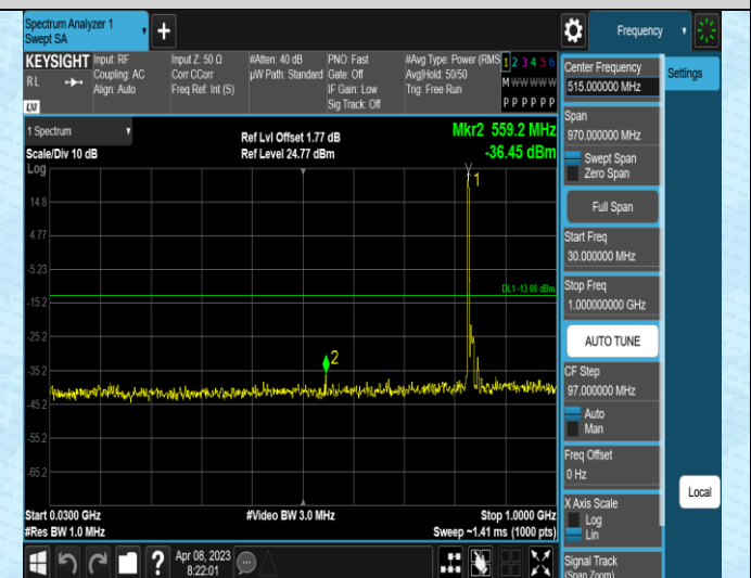
Band5-10MHz-16QAM-20600-1RB#0-Range1:30~1000
