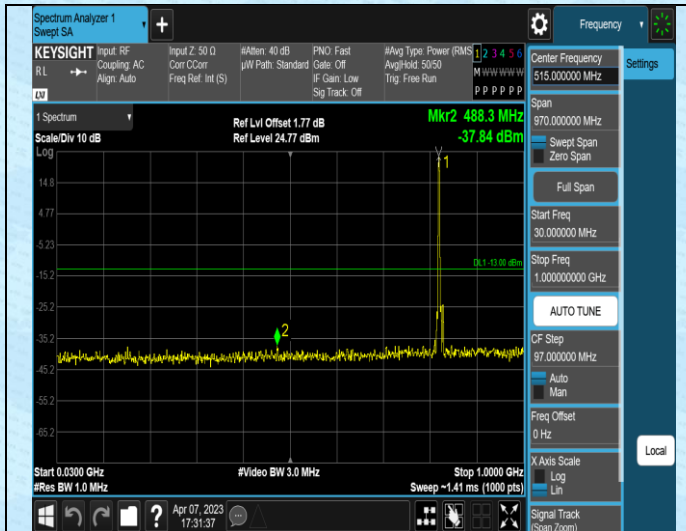
Band5-5MHz-16QAM-20525-1RB#0-Range1:30~1000M Hz
