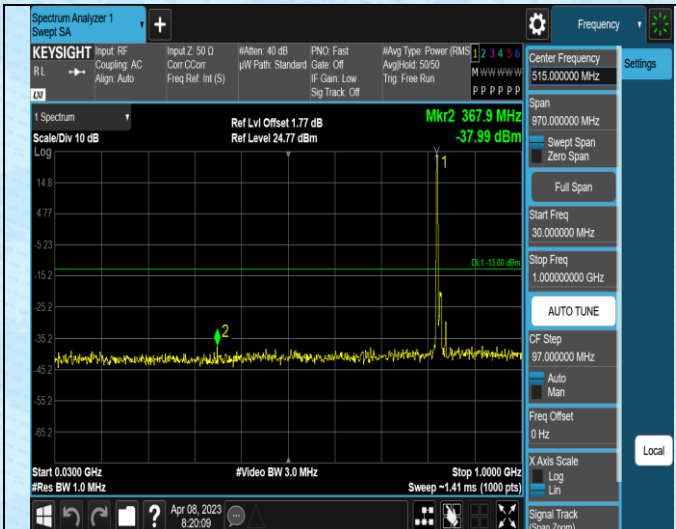
Band5-10MHz-16QAM-20525-1RB#0-Range1:30~1000
