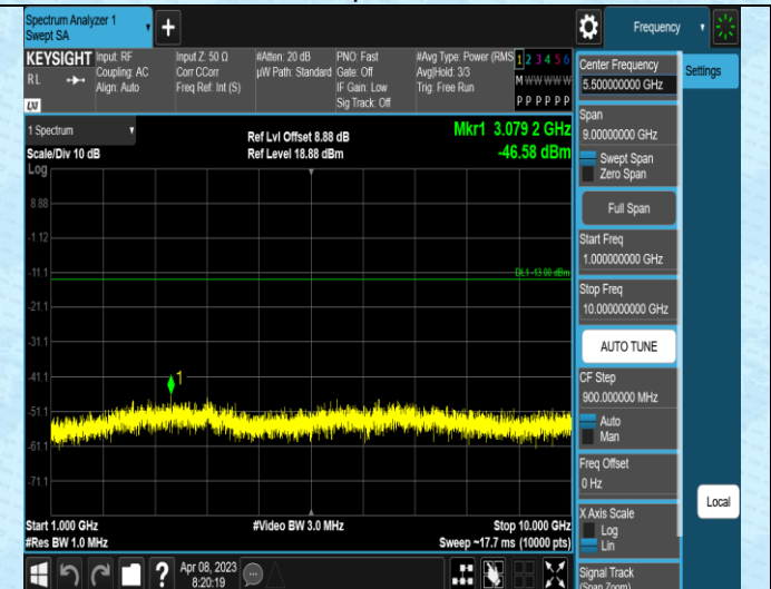
Band5-10MHz-16QAM-20525-1RB#0-Range2:30~1000
