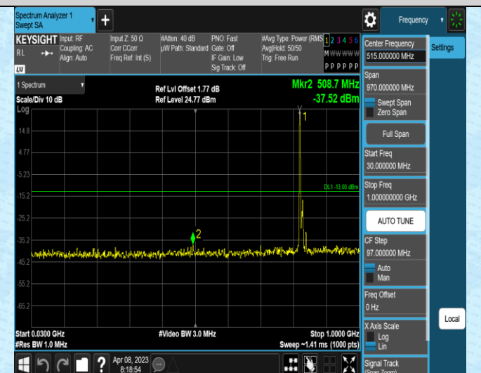
Band5-10MHz-QPSK-20525-1RB#0-Range1:30~1000M
