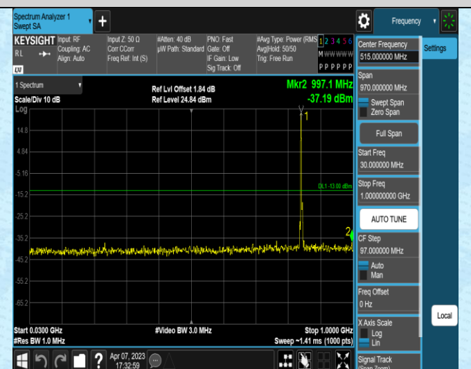
Band5-5MHz-16QAM-20425-1RB#0-Range1:30~1000MHz
