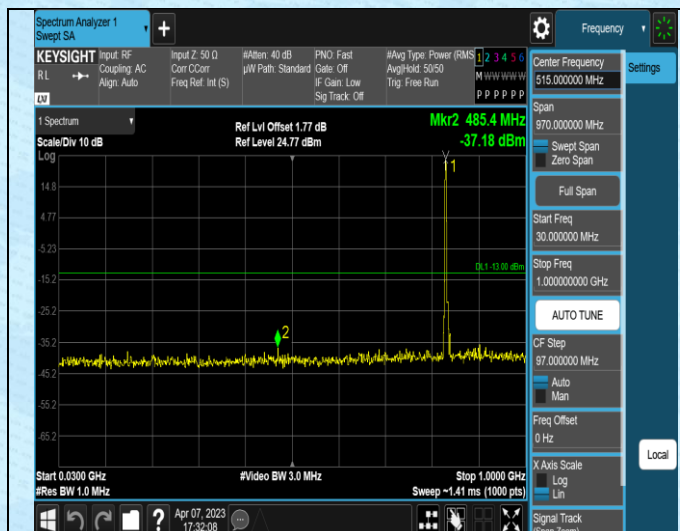
Band5-5MHz-QPSK-20625-1RB#0-Range2:30~1000MH
