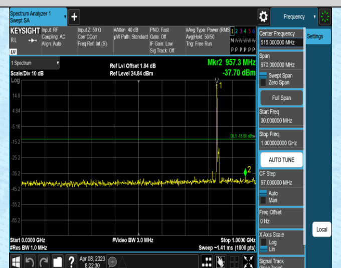
Band5-10MHz-16QAM-20450-1RB#0-Range1:30~1000
