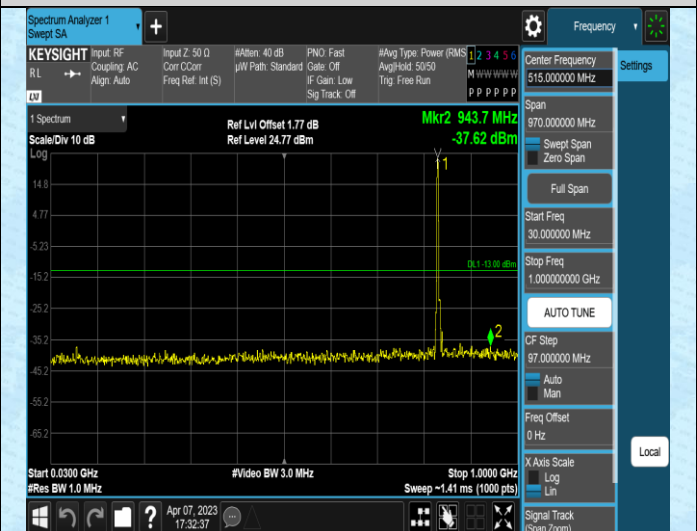
Band5-5MHz-16QAM-20625-1RB#0-Range1:30~1000M Hz
