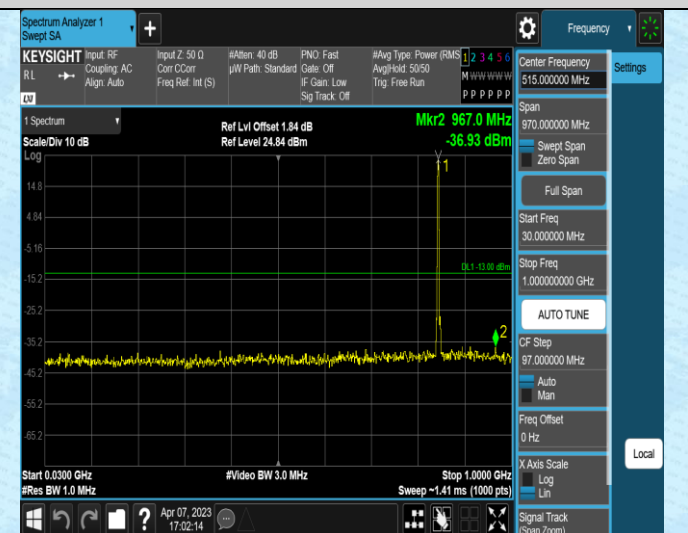
Band5-1.4MHz-16QAM-20407-1RB#0-Range1:30~1000 MHz
