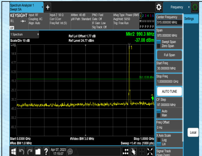
Band5-3MHz-16QAM-20525-1RB#0-Range1:30~1000M
