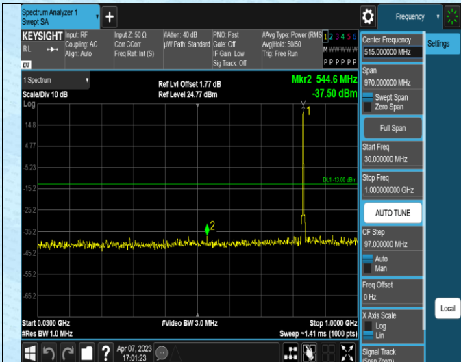
Band5-1.4MHz-QPSK-20643-1RB#0-Range2:30~1000 MHz
