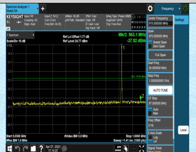
Band5-3MHz-QPSK-20525-1RB#0-Range1:30~1000MH
