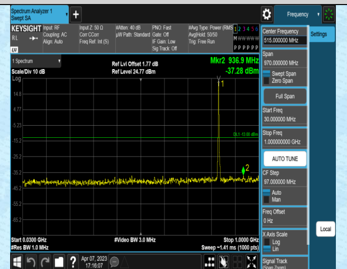
Band5-3MHz-16QAM-20635-1RB#0-Range1:30~1000M
