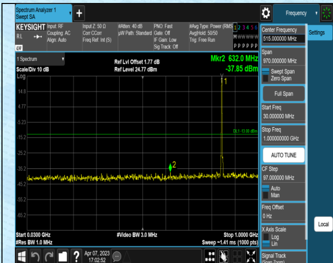
Band5-3MHz-QPSK-20415-1RB#0-Range1:30~1000MH
