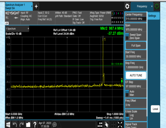
Band5-5MHz-QPSK-20525-1RB#0-Range1:30~1000MH
