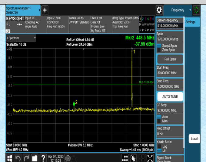
Band5-3MHz-16QAM-20415-1RB#0-Range1:30~1000M
