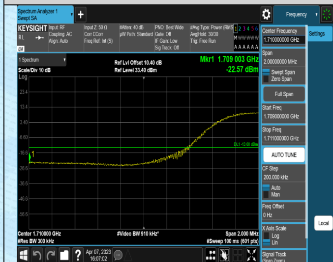
Band4-15MHz-QPSK-20025-75RB#0
