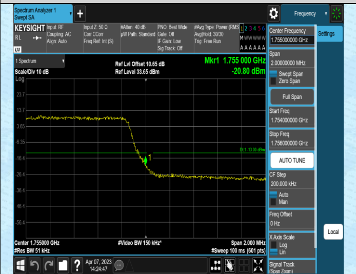
Band4-5MHz-QPSK-20375-25RB#0
