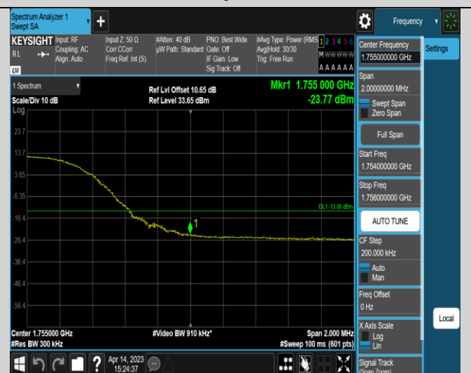
Band4-20MHz-QPSK-20300-100RB#0
