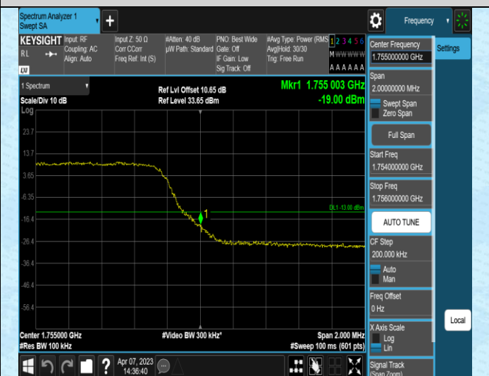
Band4-5MHz-16QAM-20375-25RB#0
