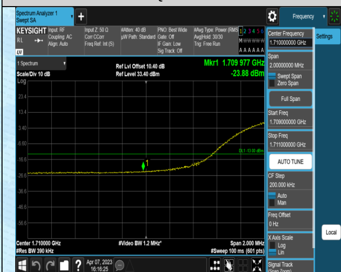
Band4-20MHz-16QAM-20050-27RB#0
