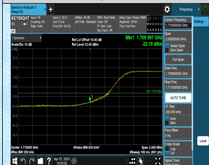
Band4-10MHz-16QAM-20000-27RB#0
