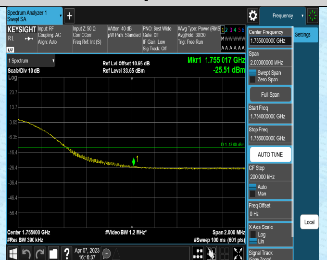
Band4-20MHz-16QAM-20300-27RB#73
