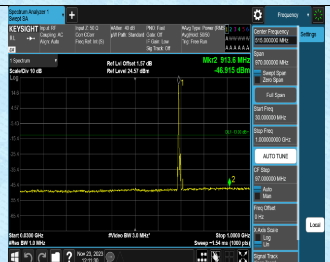
Band12-10MHz-QPSK-23095-1RB#0-Range1:30~1000 MHz
