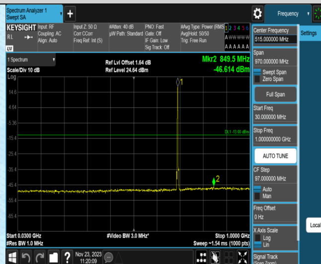
Band12-1.4MHz-QPSK-23095-1RB#0-Range2:30~1000
