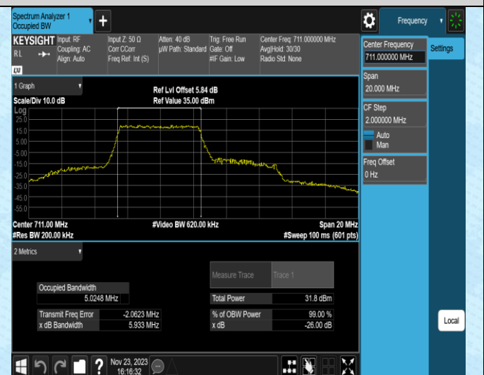
Band12-10MHz-16QAM-23130-27RB#0
