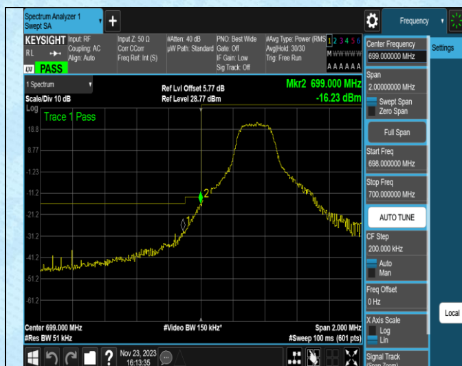
Band12-5MHz-QPSK-23155-1RB#24
