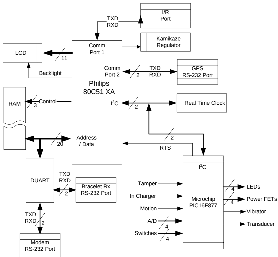
Figure 2 –SMART Active Tracking device block diagram
