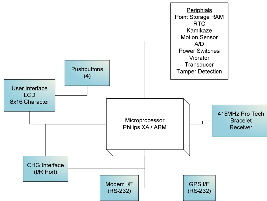
Figure 1 – High level SMART Active Tracking device block diagram
