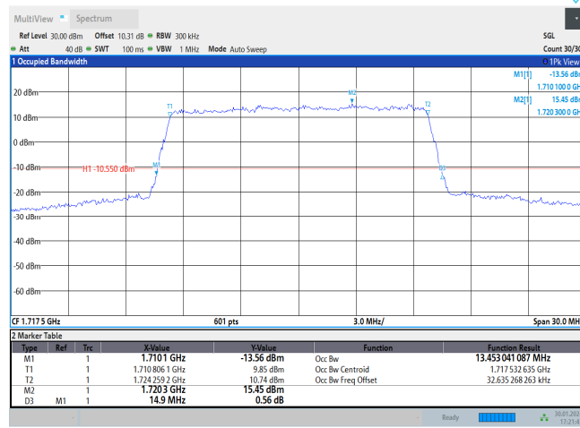
Band66-15MHz-QPSK-132322-75RB#0
