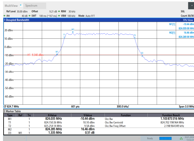
Band5-1.4MHz-QPSK-20525-6RB#0
