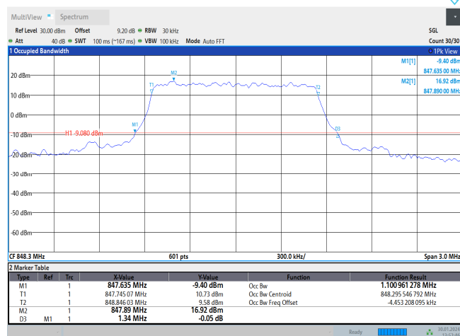
Band5-1.4MHz-QPSK-20643-6RB#0
