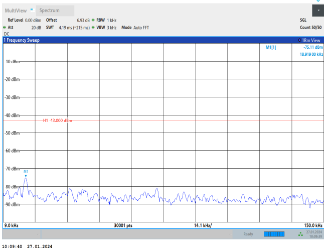
Band4-1513-4-0.009~0.15MHz
