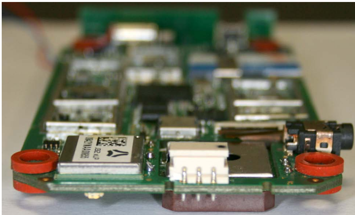
Top view 7
