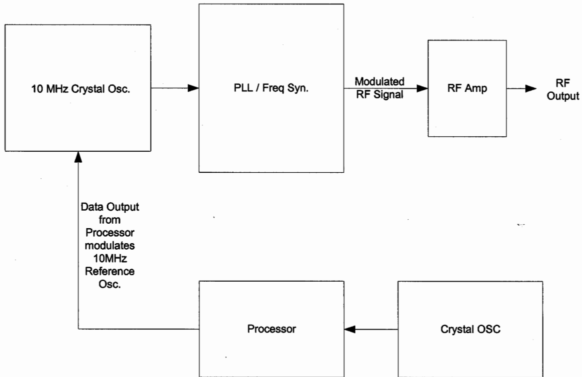
Bracelet Transmitter Block Diagram
