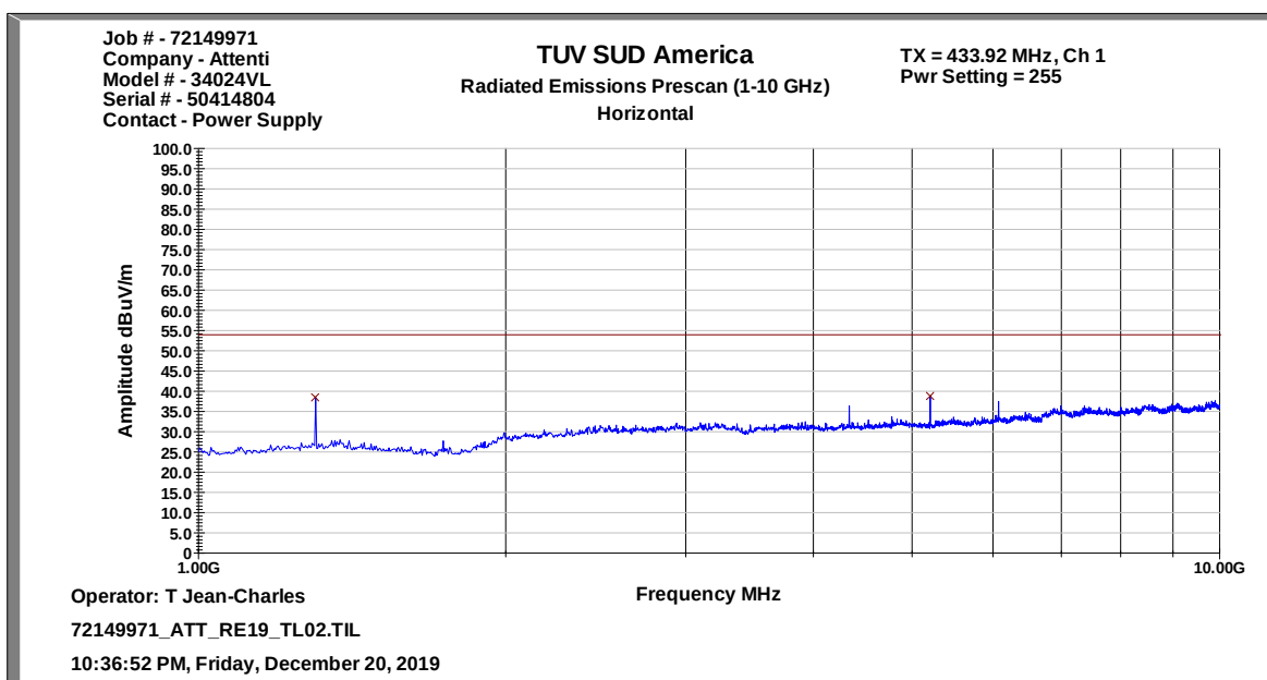
Figure 2.3.7-4: Radiated Emissions Results – 1 GHz – 10 GHz – Horizontal Polarization - Channel 1
