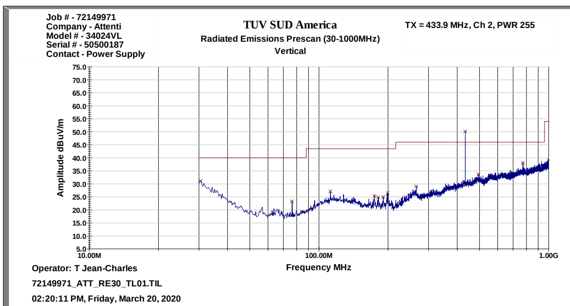
Figure 2.3.7-8: Radiated Emissions Results – 30 MHz – 1 GHz – Vertical Polarization - Channel 2
