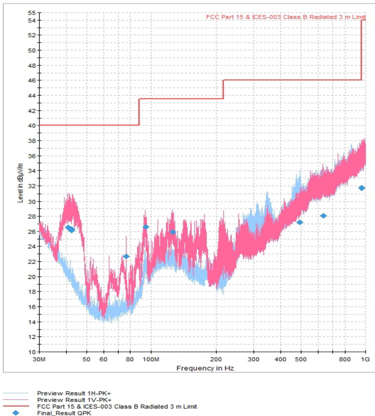
Figure 2.2.8-1 - Graphical Results 30 MHz to 1 GHz - Horizontal and Vertical Polarity
