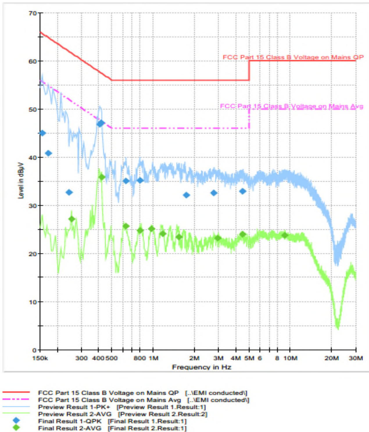
Figure 2.1.8-1 - Graphical Results - AC Mains Composite Line and Neutral Plot
