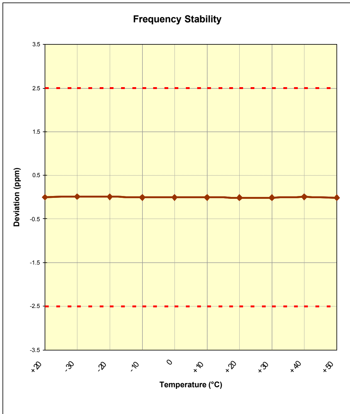
Plot 6-27. Frequency Stability Graph (PCS WCDMA Mode – Ch. 9400)
