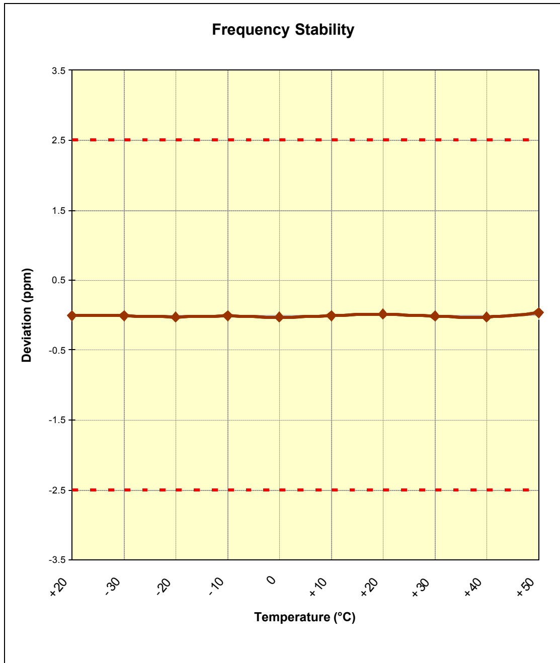
Plot 6-21. Frequency Stability Graph (Cellular GSM Mode – Ch. 190)
