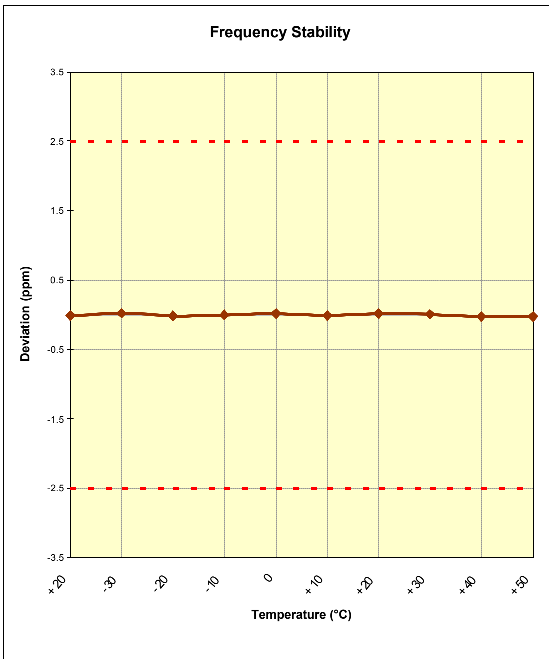
Plot 6-23. Frequency Stability Graph (Cellular WCDMA Mode – Ch. 4183)
