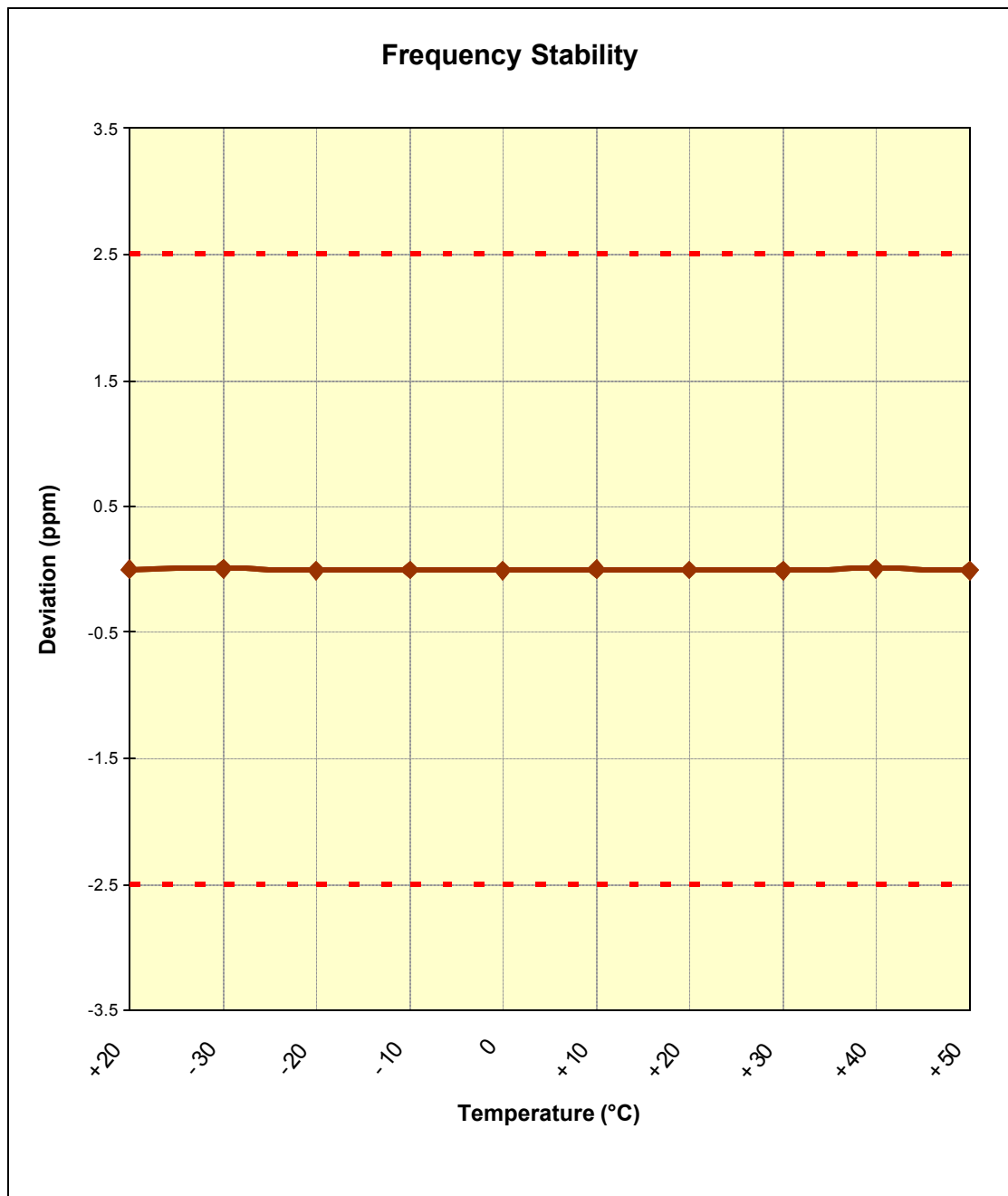
Plot 6-25. Frequency Stability Graph (PCS GSM Mode – Ch. 661)
