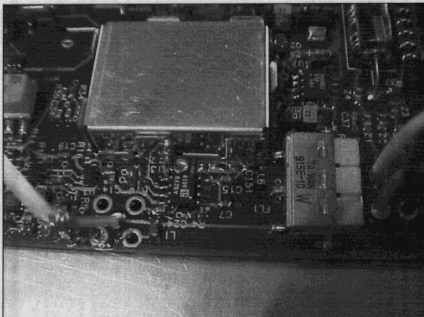
Photo 5: RF BPF Area, Top View, Shield Cover in Place, PROX-100, Modified
