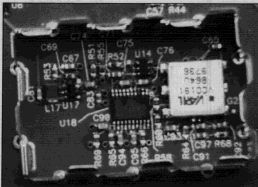
Photo 12: RF Shield Removed
