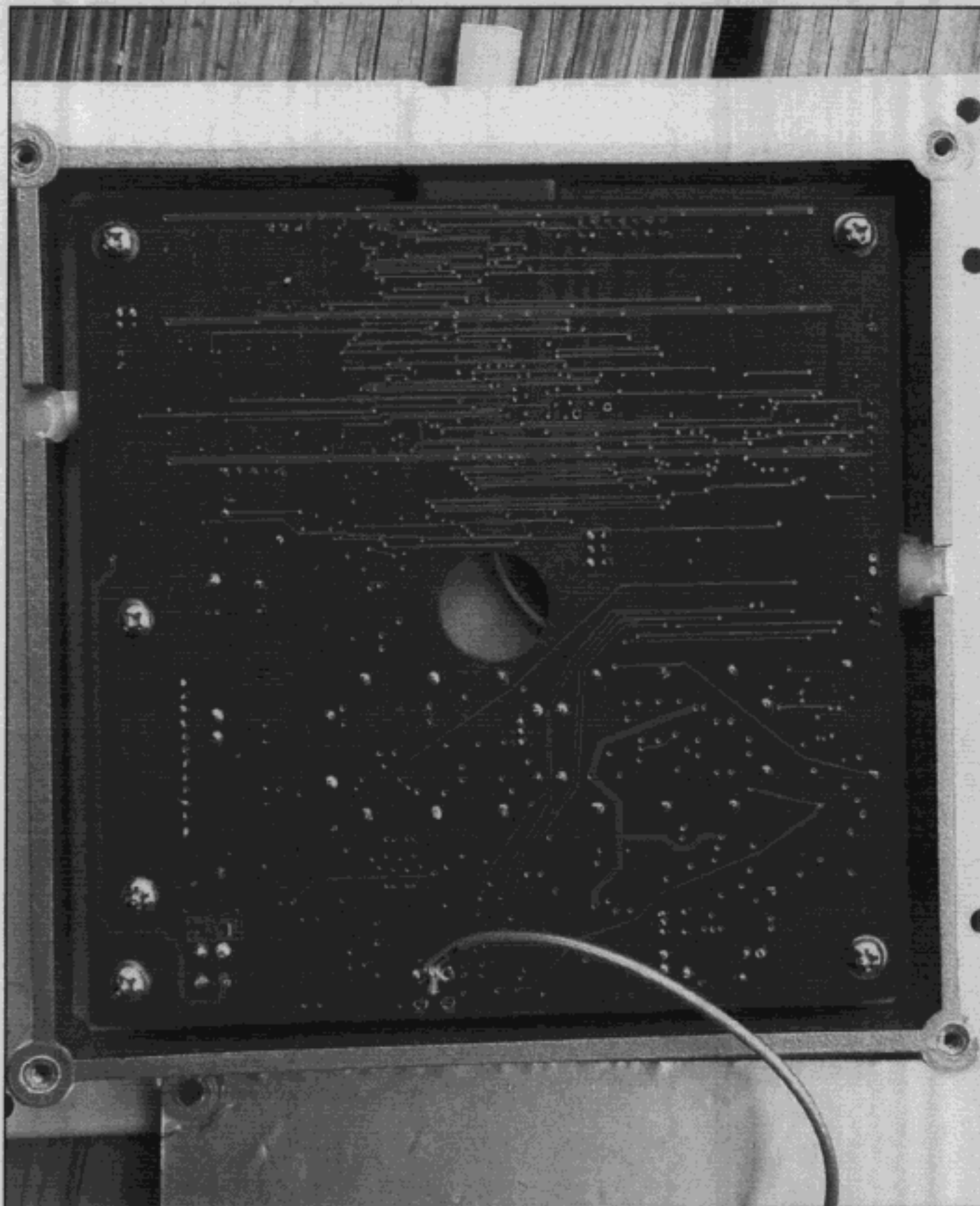
Photo 10: PROX-100, Horizontal, Wall Mount, PCB, Circuit Side
