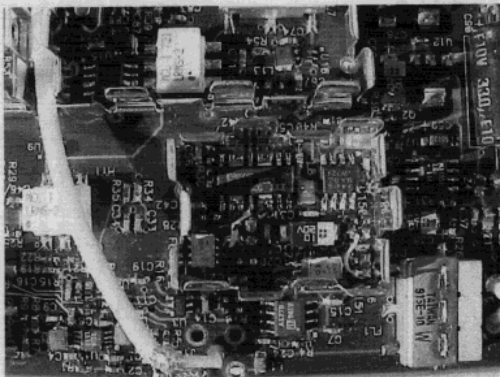
Photo 4: RF PA/BPF Area, Top View, Shield Covers Removed, PROX-100, Modified
