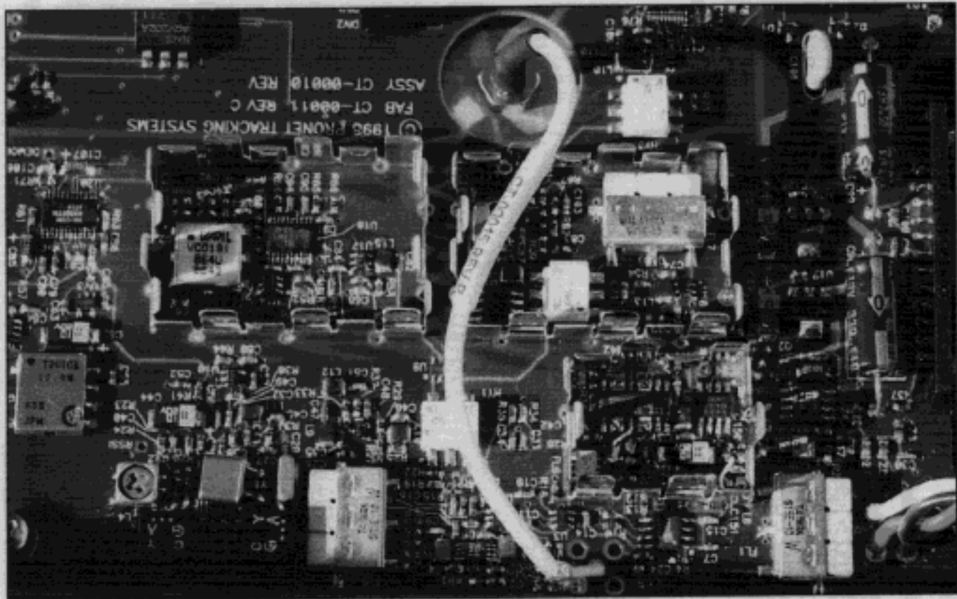
Photo 3: RF Area, Top View, Shield Covers Removed, PROX-100, Modified
