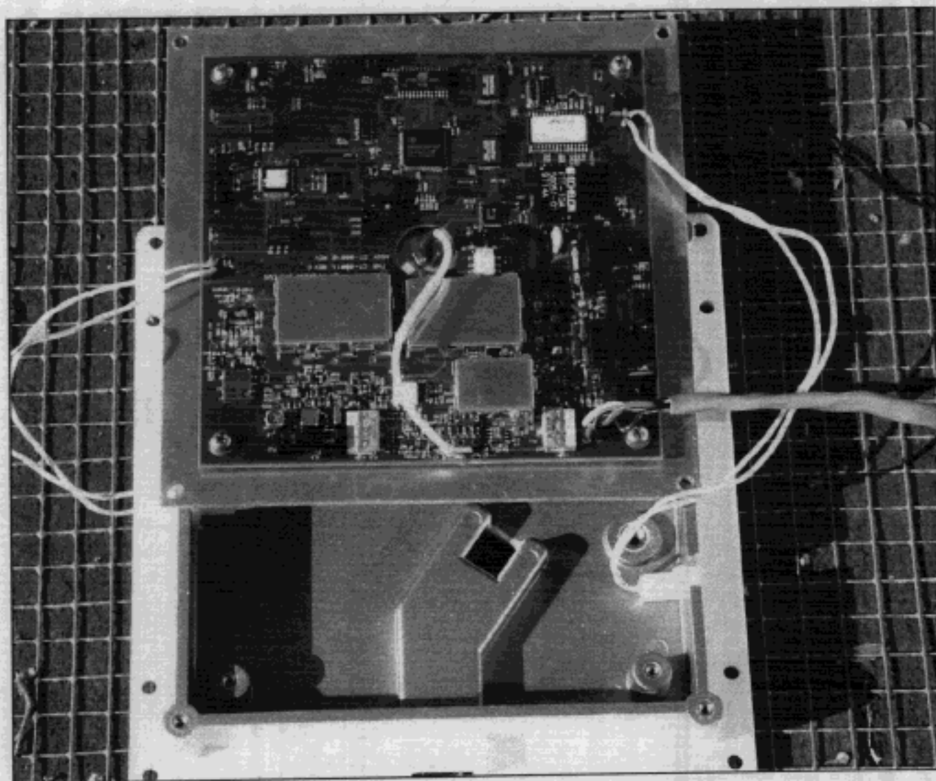
Photo 1: RF Board, Top View, PROX-100, Modified
