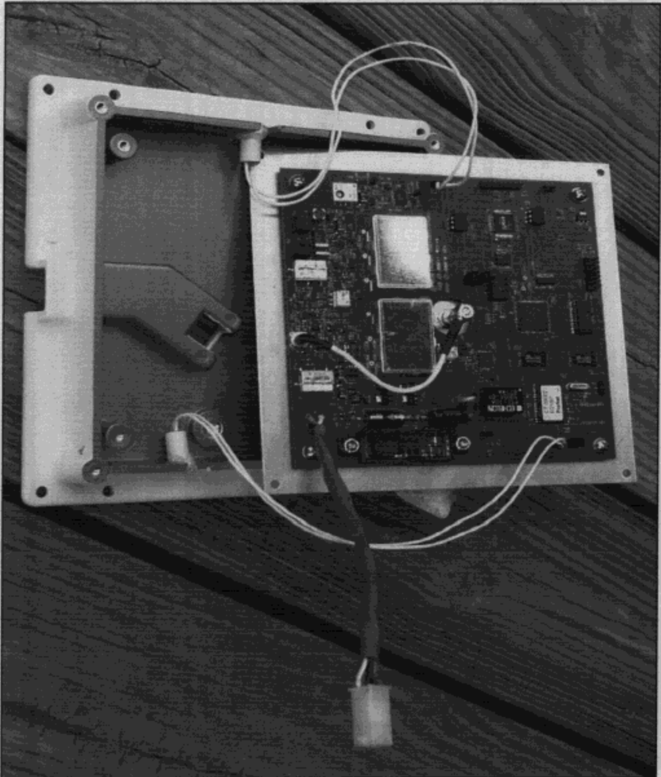
Photo 3: PROX-100, Vertical, Ceiling Mount, Exploded View
