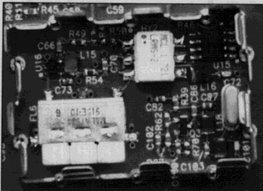
Photo 11: RF Shield Removed
