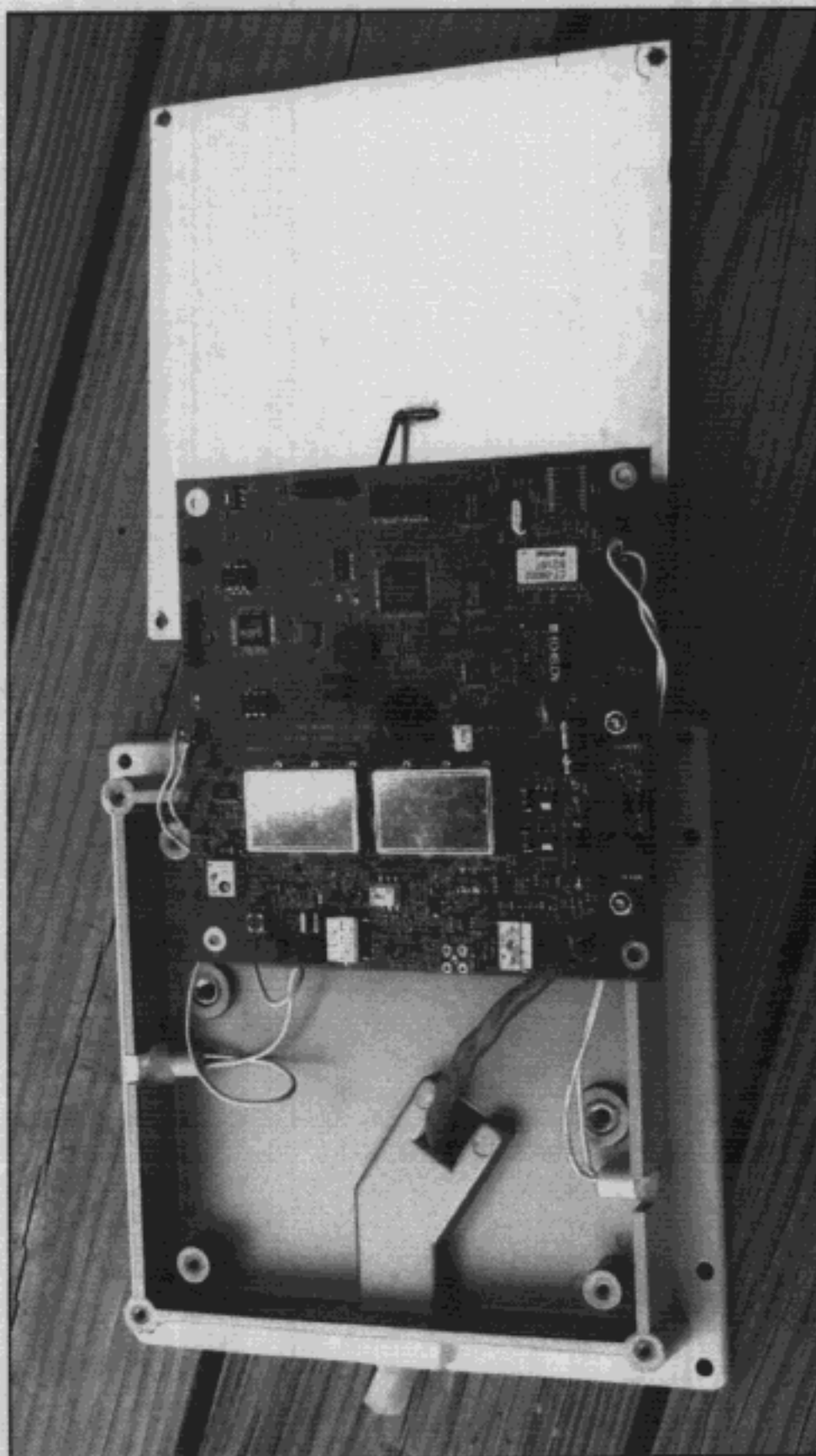
Photo 8: PROX-100, Horizontal, Wall Mount, Exploded View
