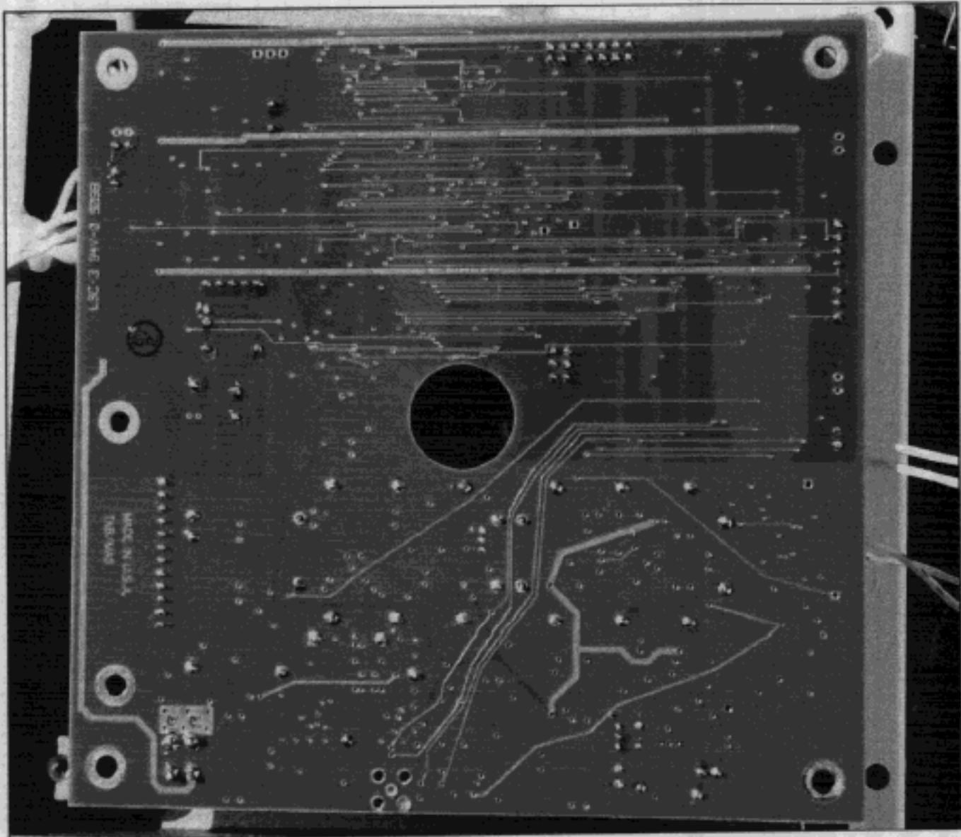
Photo 2: RF Board, Bottom View, PROX-100, Modified
