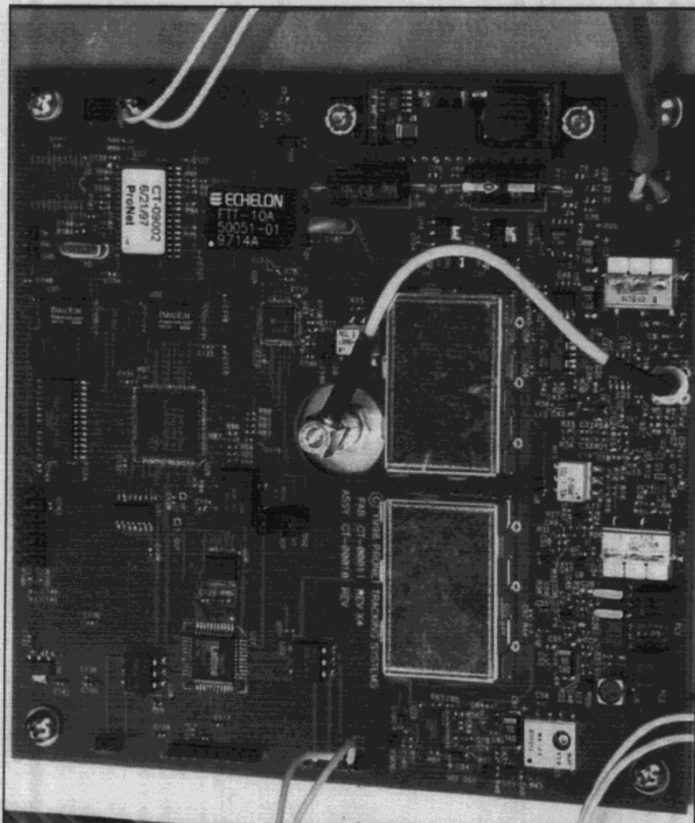
Photo 4: PROX-100, Vertical, Ceiling Mount, , PCB, Top View
