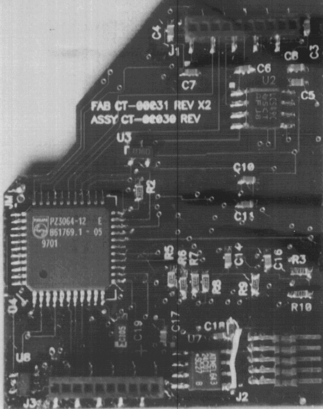
Photo 9: Digital Board, Bottom View, PAD-1000
