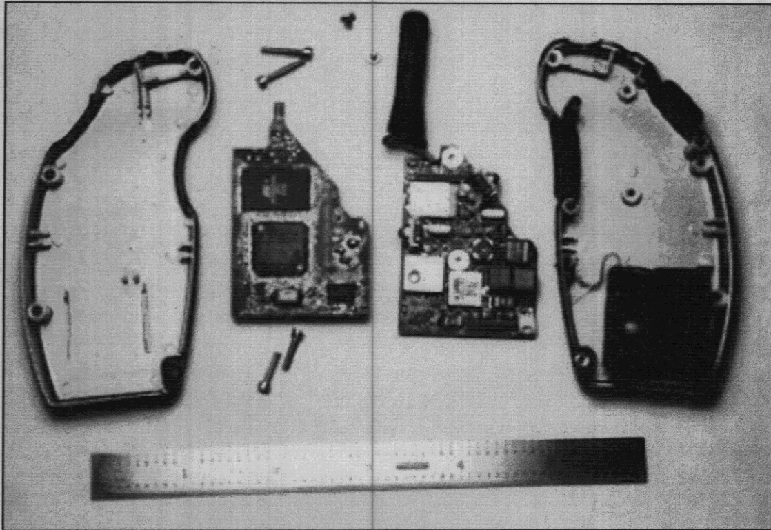
Photo 2: Exploded View, Pad-1000
