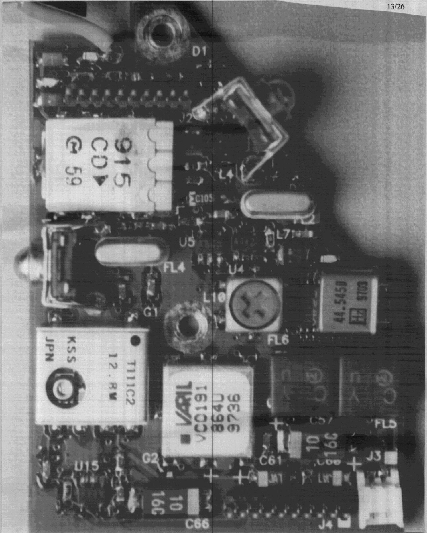
Photo 6: RF Board, Outside of Enclosure, PAD-1000
