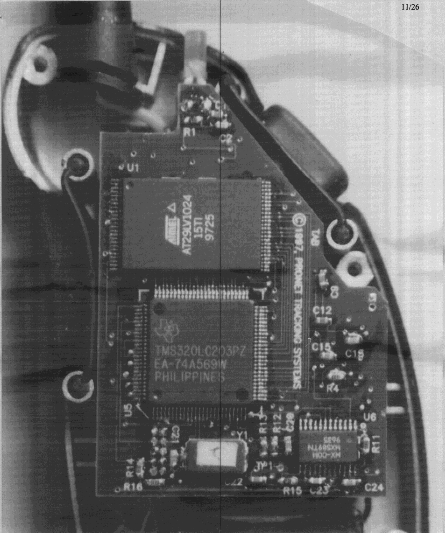
Photo 4: Detail View, Board Stack, PAD-1000
