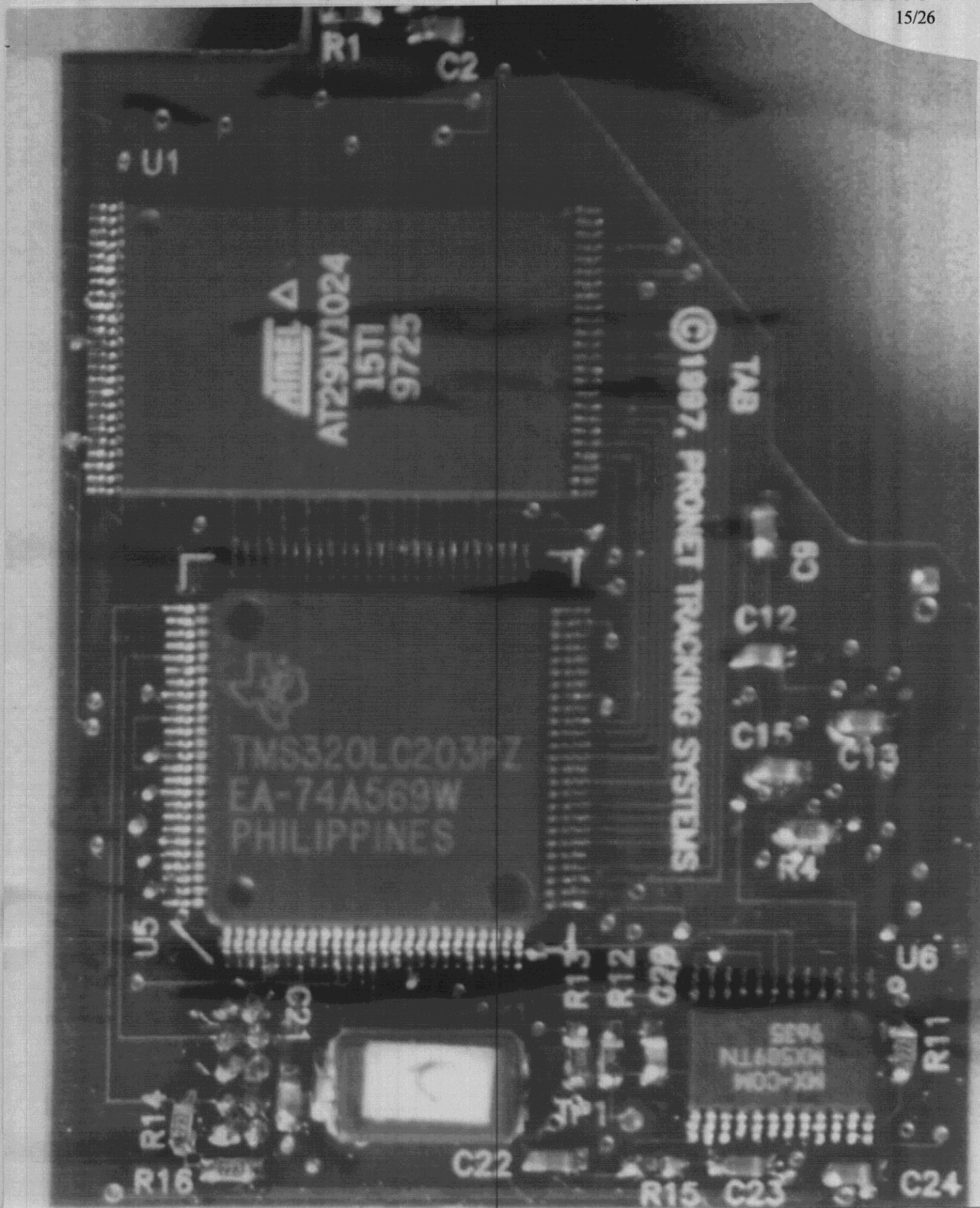
Photo 8: Digital Board, Top View, PAD-1000
