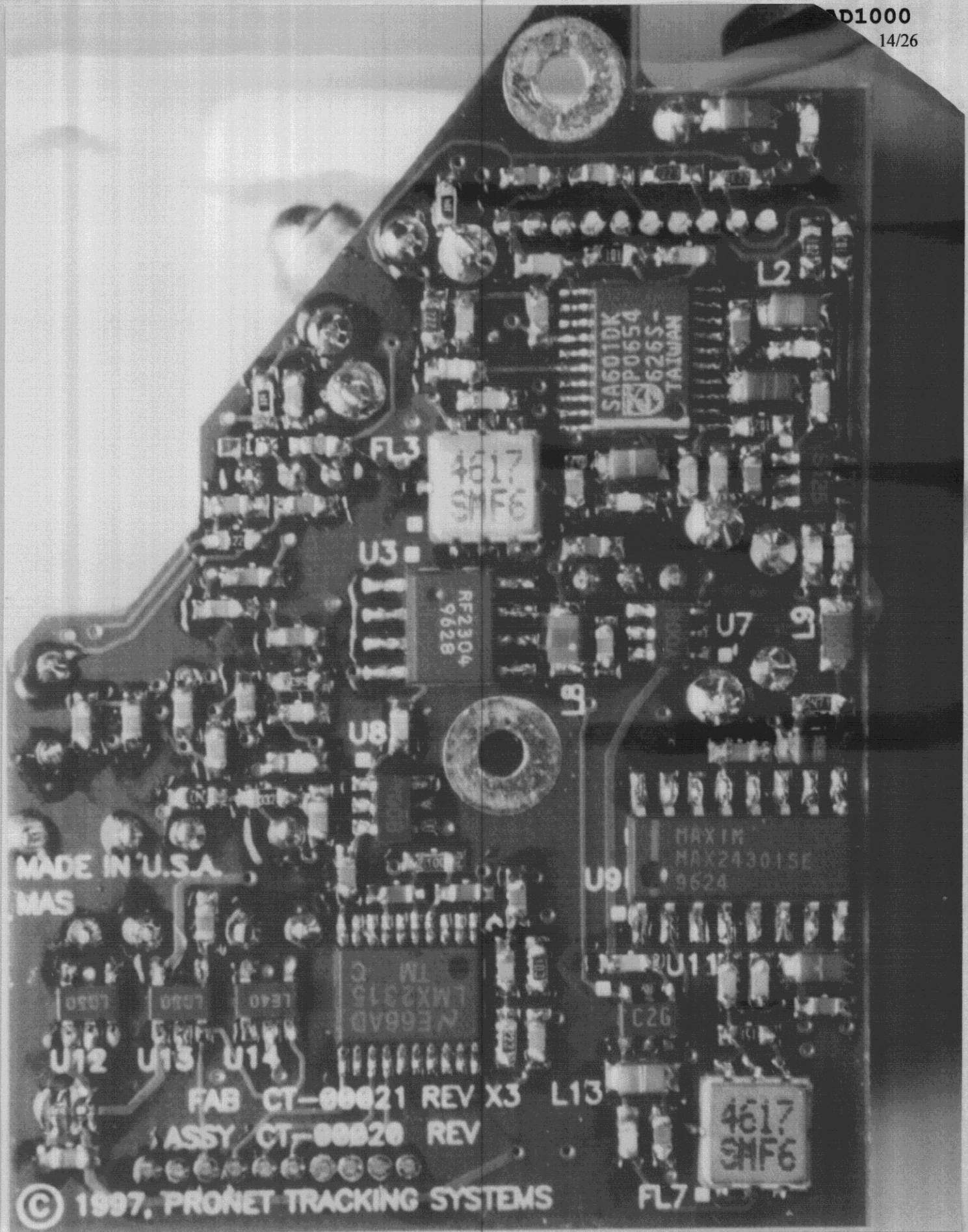
Photo 7: RF Board, Bottom View, PAD-1000
