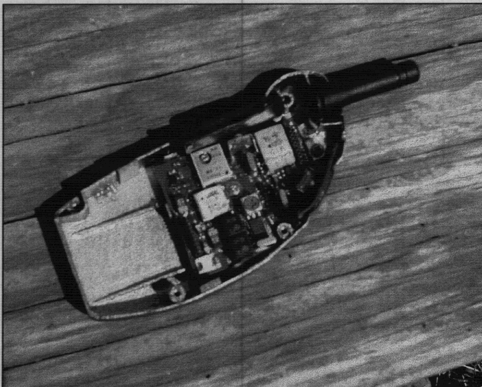
Photo 3: Interior View, Battery Removed, PAD-1000
