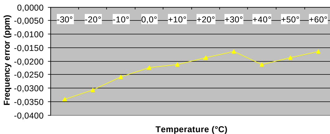
Frequency Error vs. Temperature
