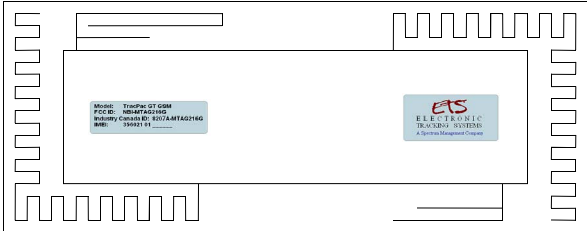
Product Label Location, TracPac GT GSM Bottom surface (non-component side)
