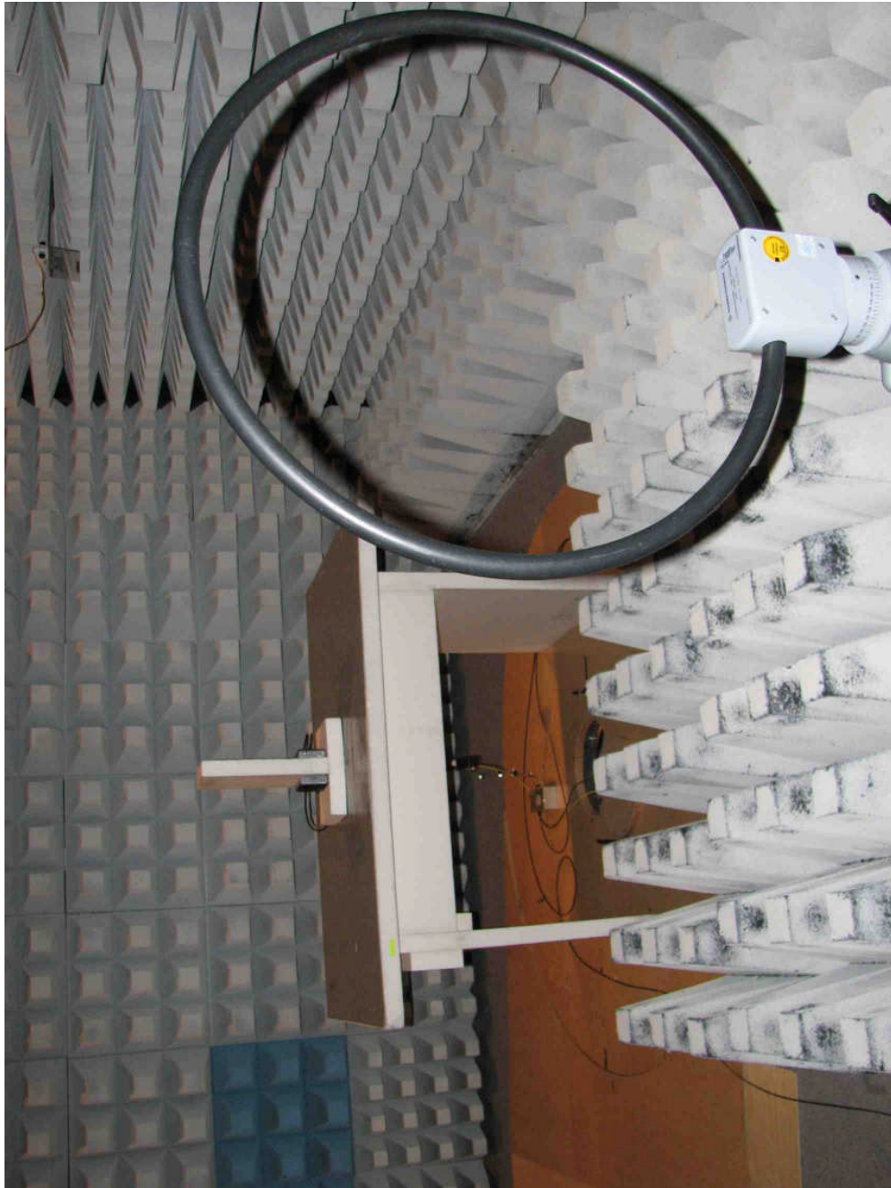
72572emi2.JPG: Test set-up preliminary radiated H-Field
