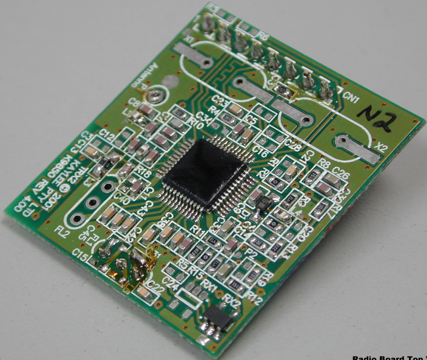
Radio Board Top View
