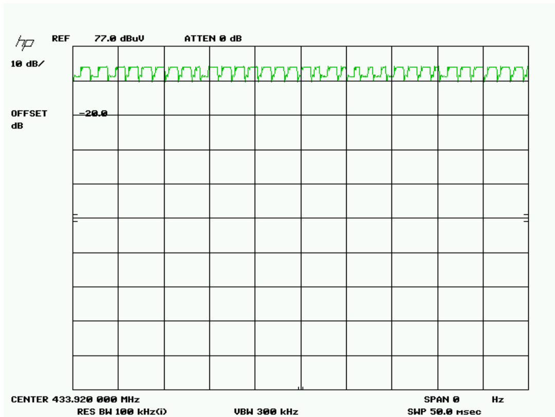
DUTY CYCLE PLOT
