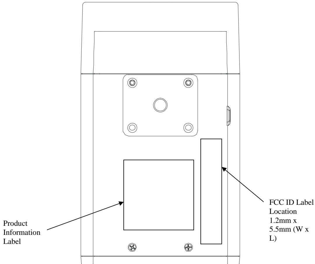
Bottom View of Network Camera: Model NF610
