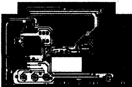
900-TPX301-10300V0 Top Routing
