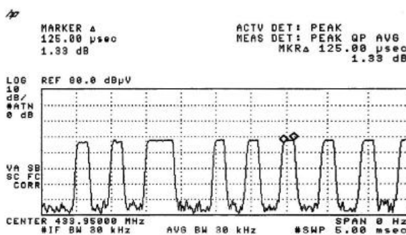
Figure C [Short Pulse]
