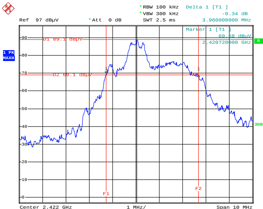
20 dB bandwidth (2422MHz)
