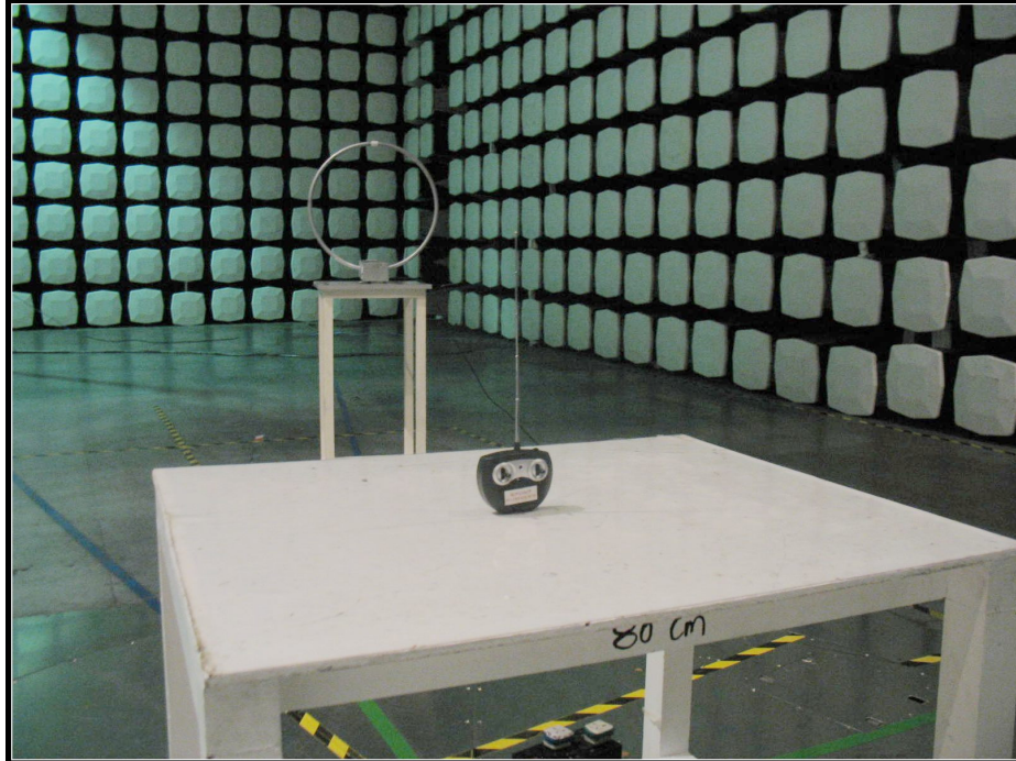
Radiated Emission & Fundamental Emission (below 30 MHz)
