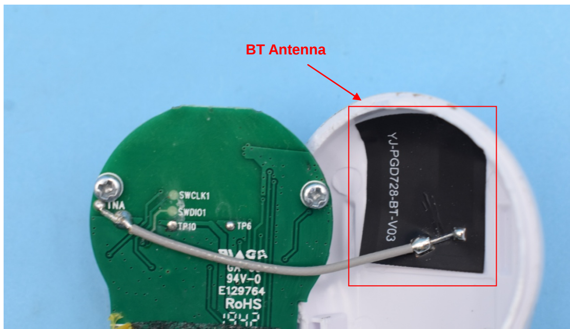
2. Antenna view
