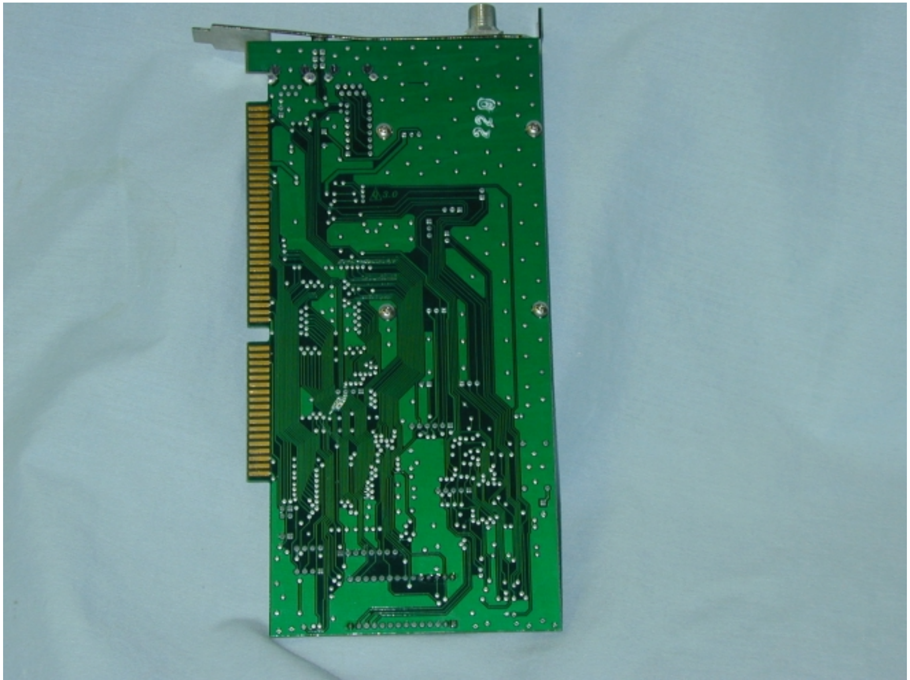
Photo 2 - PC Card Trace Side
