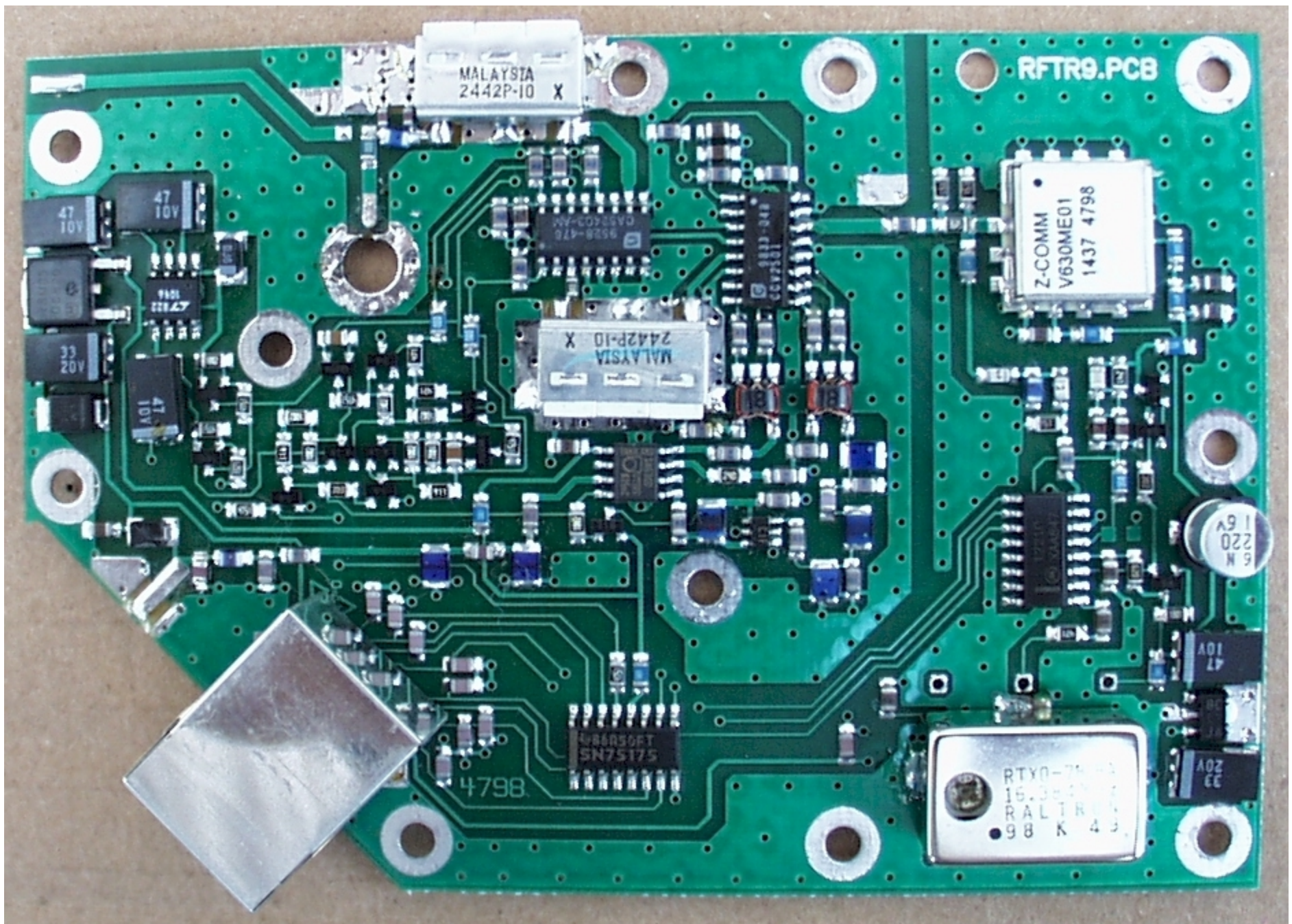
Photo 6 - Antenna/RF PCB Component Side
