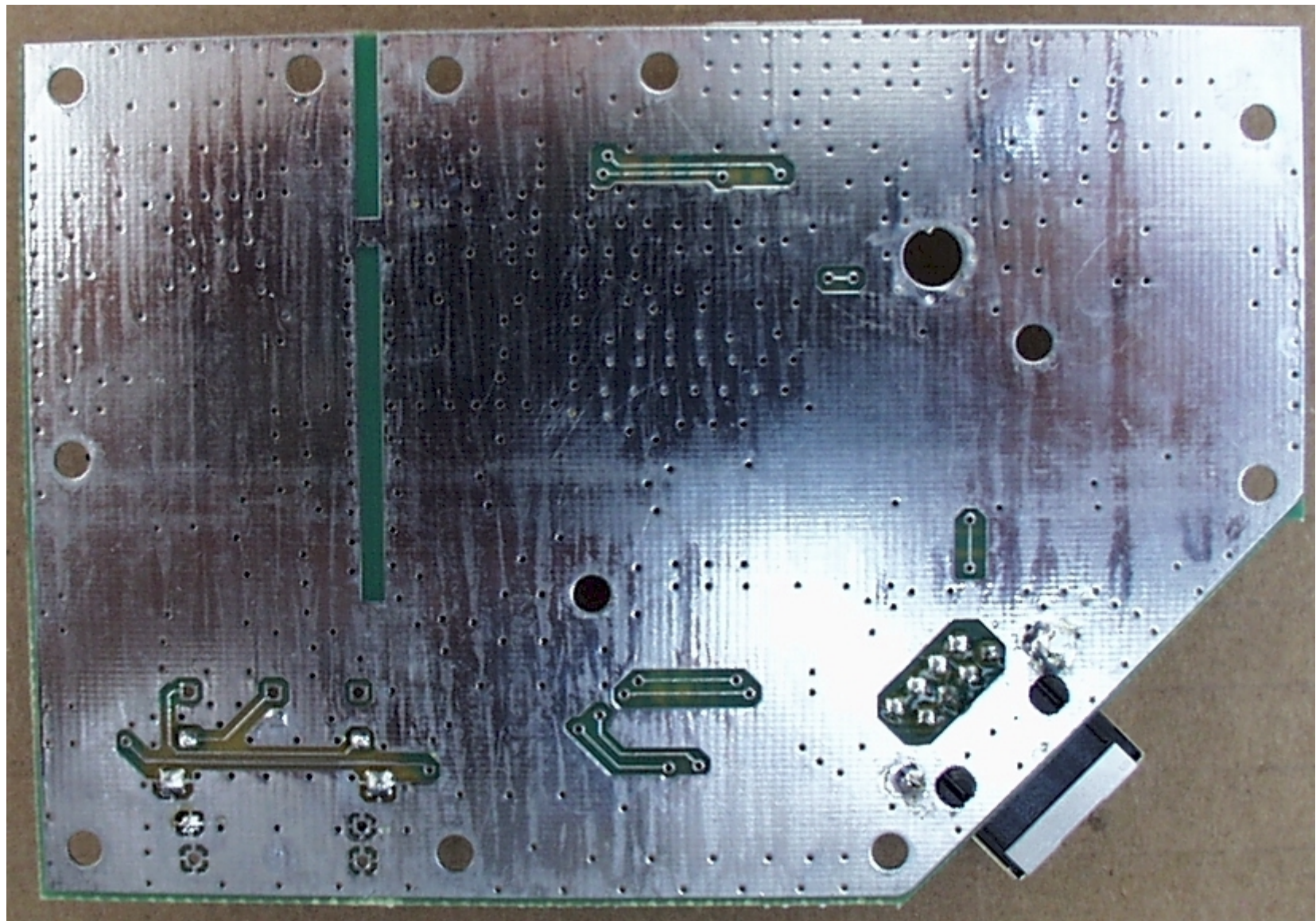
Photo 7 - RF/Antenna PCB Trace Side
