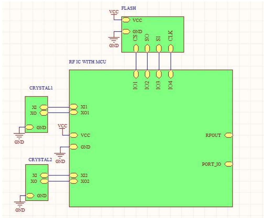
Figure1 Structure Diagram
