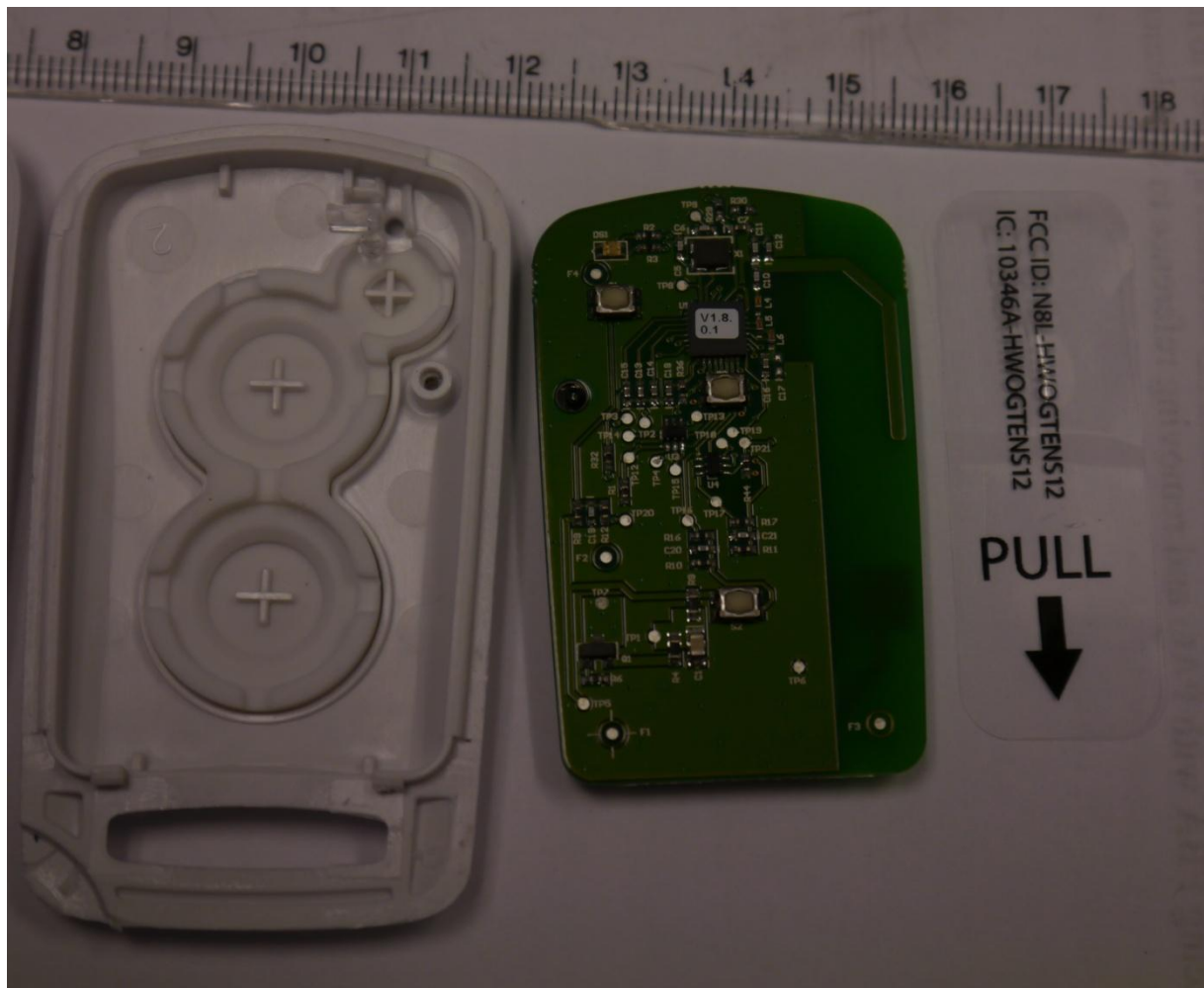
Back side of PCB and inside cover
