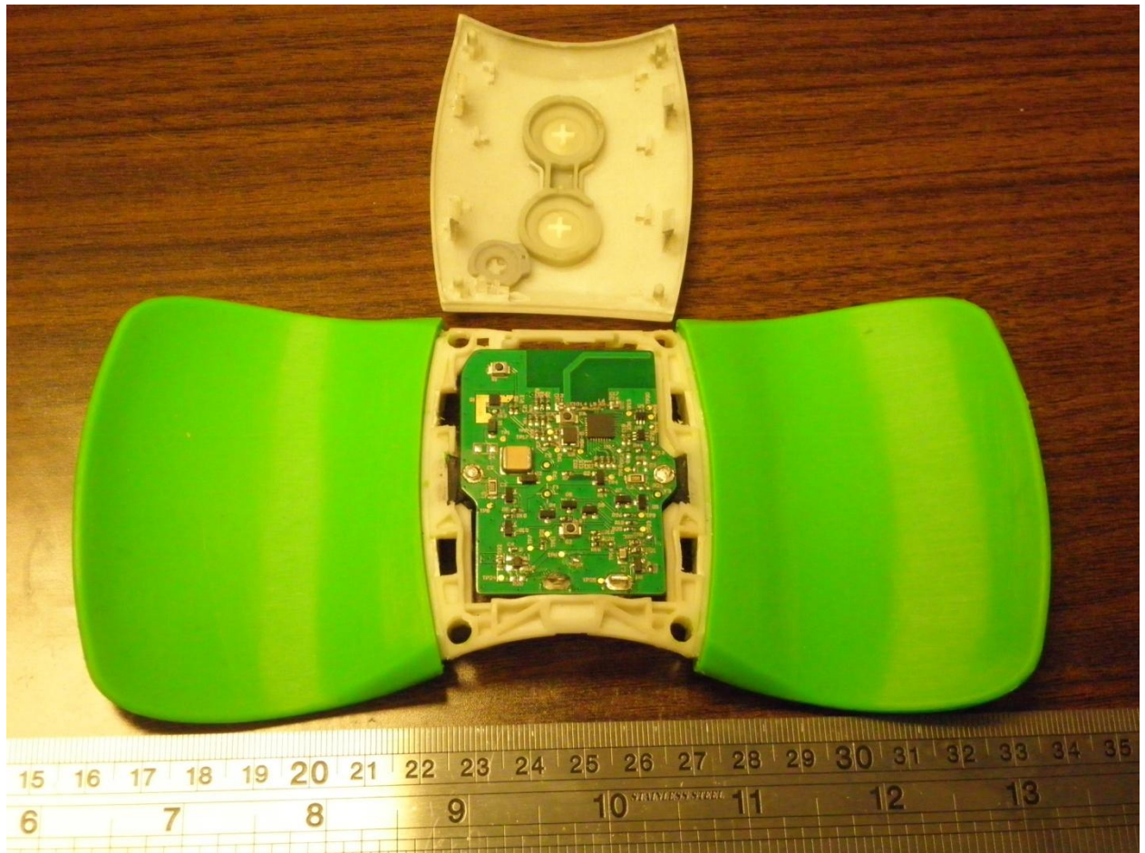
Front side top cover removed
