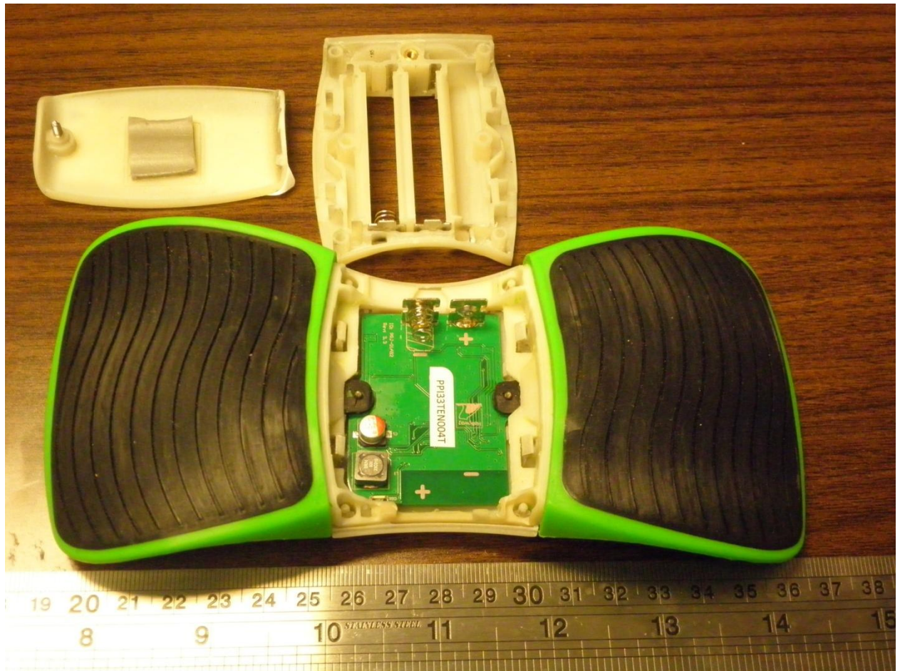
Back side: Battery compartment removed (back side of PCB)
