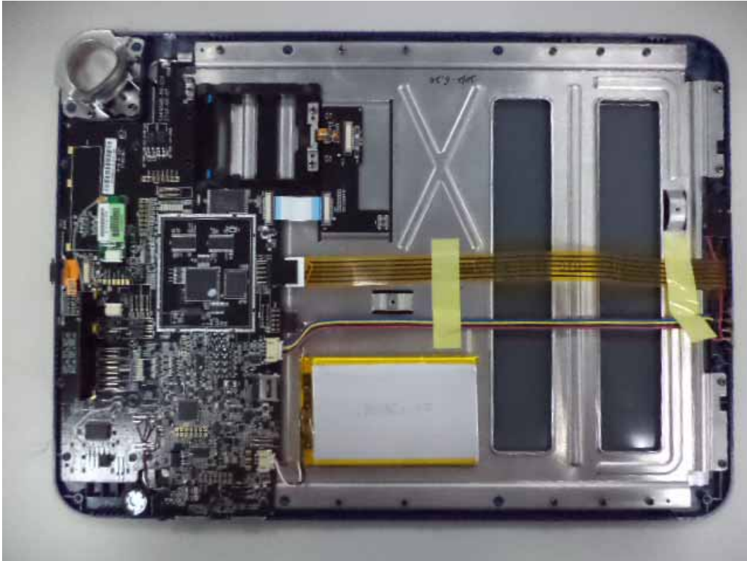
Figure 4 Internal View (Control Board, Front View)
