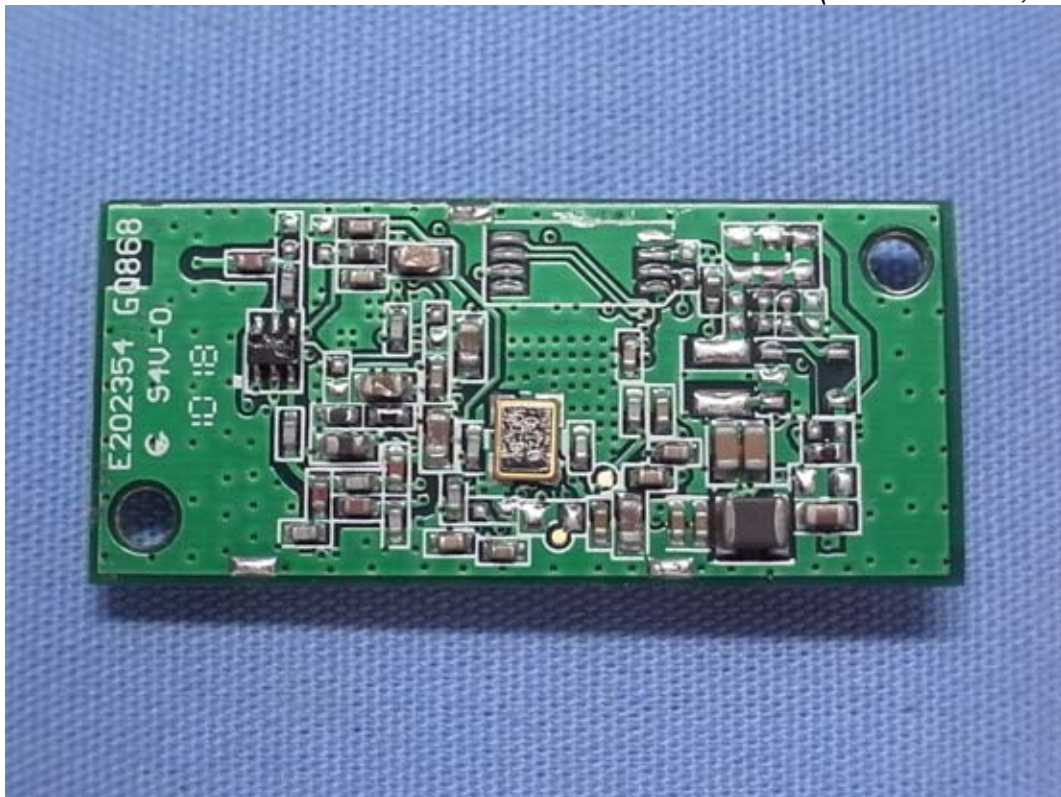
Figure 17 Internal View (WI-FI Module, Back View)
