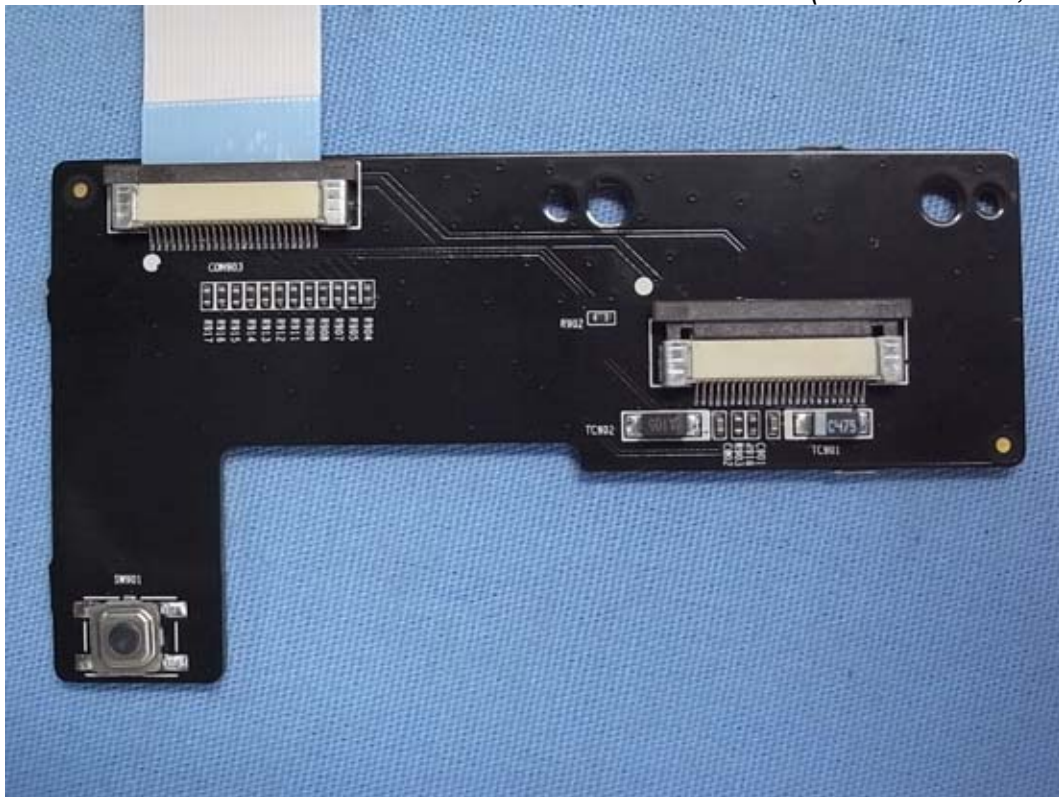
Figure 9 Internal View (Control Board, Front View)
