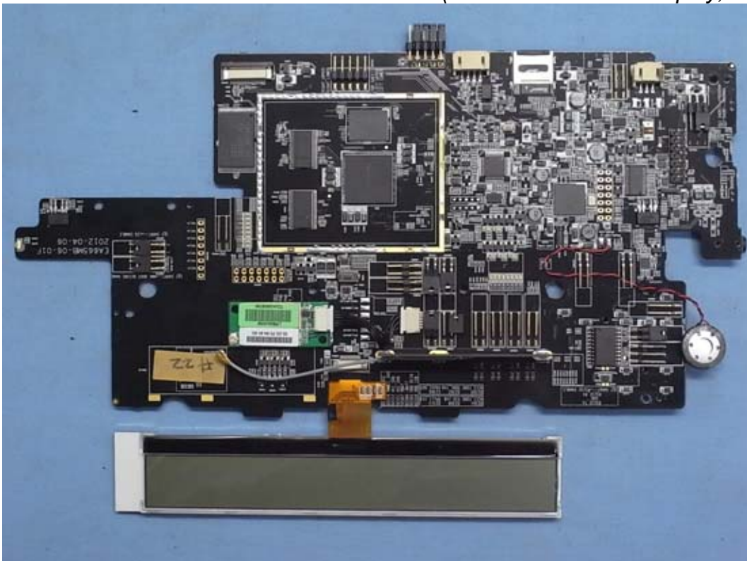
Figure 12 Internal View (Main Board & LCD Display, Front View)
