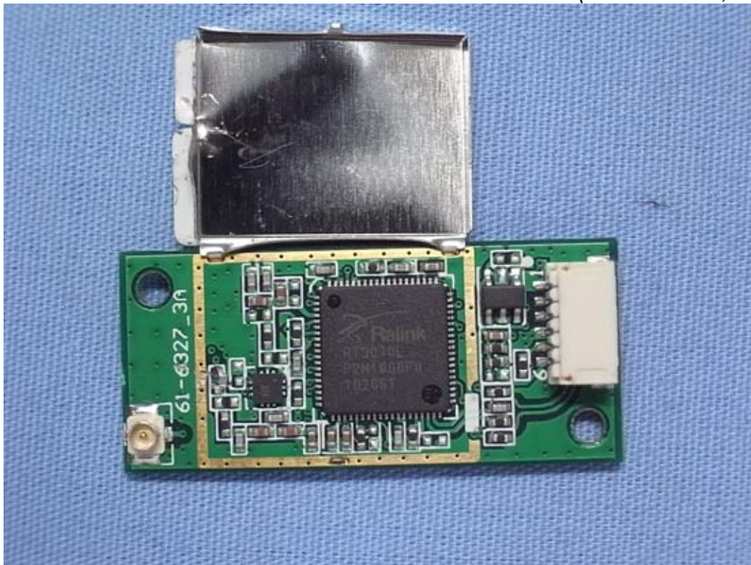
Figure 15 Internal View (WI-FI Module, Front View)
