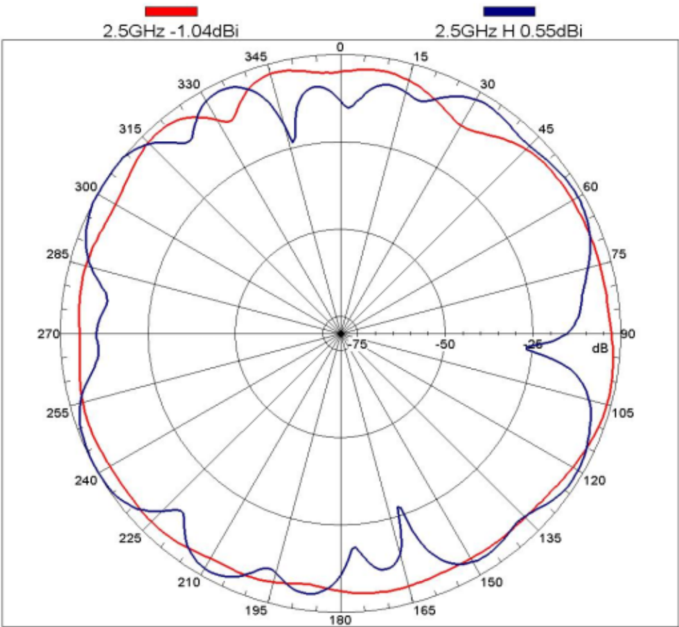
Far-field amplitude of EAL-20 2.4~2.5G L-H Patten CO.nsi
