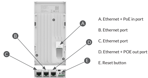
FIGURE 2: RAP630W-311G / 211G AP Ports on Bottom Panel.
