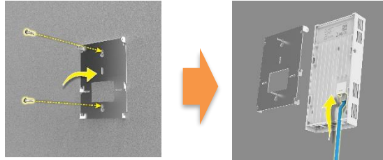
FIGURE 10 Fit into slots on the bottom of the EWW631-B1
