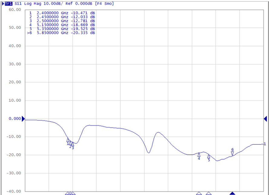
Figure 2 Return Loss
