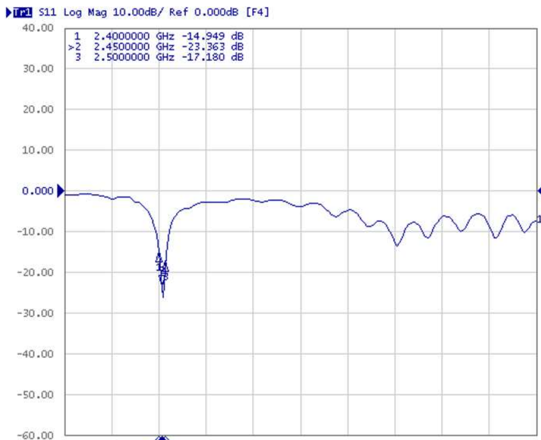
Figure 2 Return Loss
