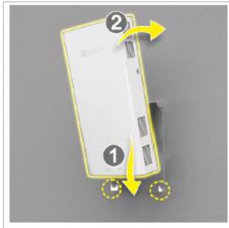
FIGURE 6: Fit into slots on the bottom of the RAP630W-311G / 211G.
