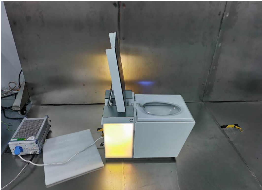
Conducted Emissions Side View
